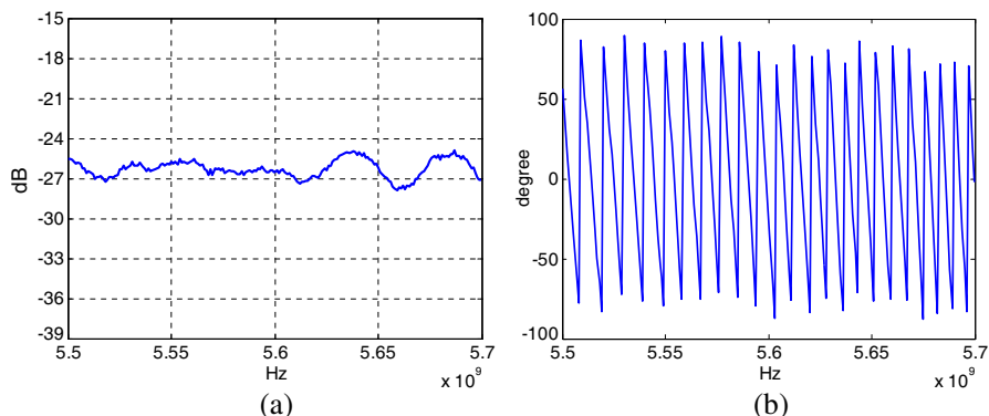
Figure 4. The frequency domain response. (a) Amplitude, (b) phase.
