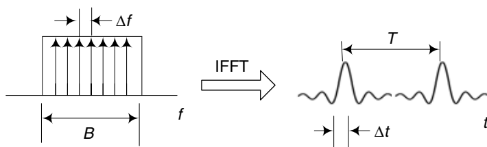
Figure 2. The frequency domain and time domain correspondence.
