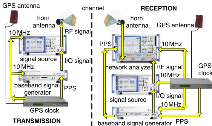
Figure 1. The diagram of the measurement system.
