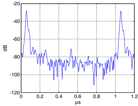
Figure 5. The time domain response.
