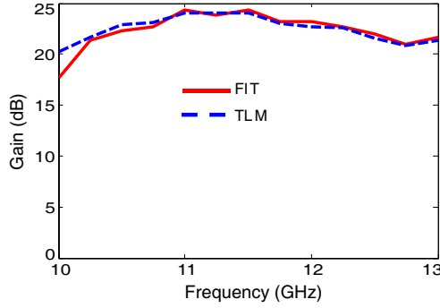
Figure 4. Gain versus frequency for 13 \times 13 planar reflectarray.
