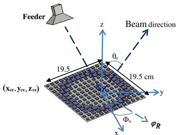
Figure 2. The geometry of DRA reflectarray.
