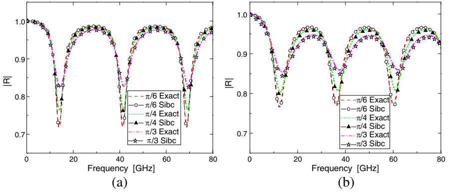
Figure 5. Magnitude of the reflection coefficient of TM plane wave at varying oblique angles. Parameters of the coating: (a) d = 1 mm, \varepsilon'_{1,r} = 30 , \sigma_1 = 1 S/m. (b) d = 2 mm, \varepsilon'_{1,r} = 10 , \sigma_1 = 0.4 S/m.
