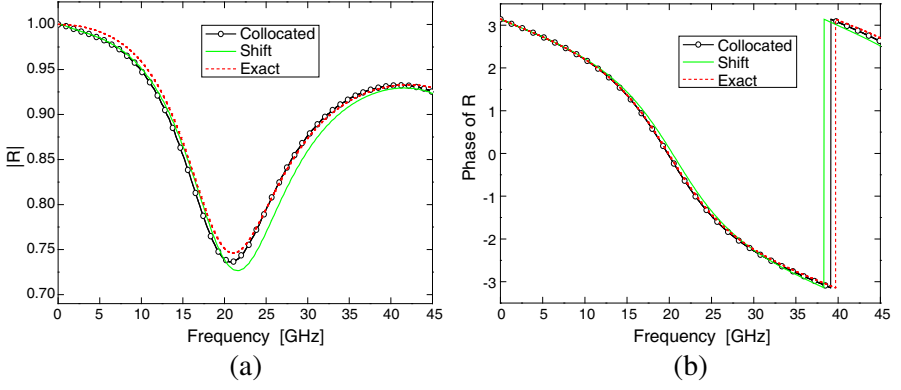
Figure 4. The reflection coefficient of TM plane wave from a coated conductor at the angle of incidence \theta = 60^\circ . Parameters of the coating: d = 1 mm, \varepsilon'_{1,r} = 15 , \sigma_1 = 1.5 S/m. (a) Magnitude. (b) Phase.
