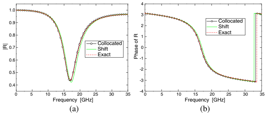
Figure 6. The reflection coefficient of TE plane wave from a coated conductor at the angle of incidence \theta = 15^\circ . Parameters of the coating: d = 1 \text{ mm} , \varepsilon'_{1,r} = 20 , \sigma_1 = 2 \text{ S/m} . (a) Magnitude. (b) Phase.
