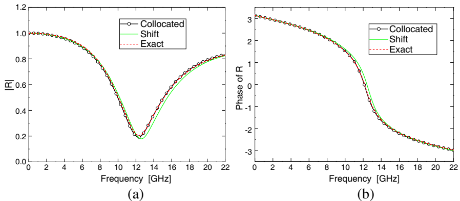
Figure 3. The reflection coefficient of TM plane wave from a coated conductor at the angle of incidence \theta = 30^\circ . Parameters of the coating: d = 2 mm, \varepsilon'_{1,r} = 10 , \sigma_1 = 2 S/m. (a) Magnitude. (b) Phase.
