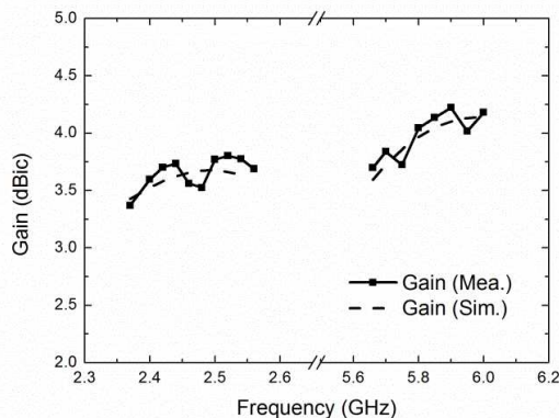
Figure 9. Simulated and measured gain.
