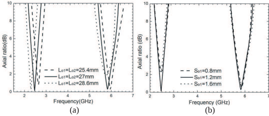
Figure 3. (a) Simulated axial ratio for different values of L_{o1} and L_{o2} . (b) Simulated axial ratio for different values of S_{o1} .
