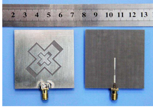
Figure 5. Photograph of the proposed antenna.
