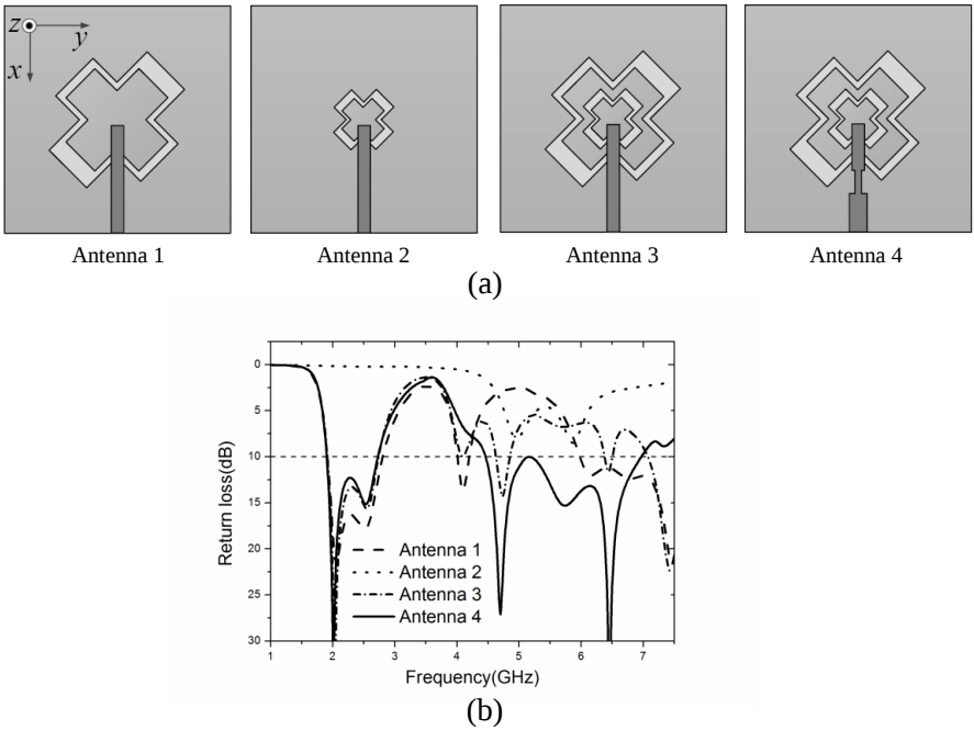
Figure 2. (a) Design evolution of the proposed antenna. (b) Corresponding simulated return losses curves.
