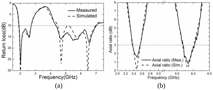
Figure 6. The simulated and measured (a) return losses, (b) axial ratios on z -axis.
