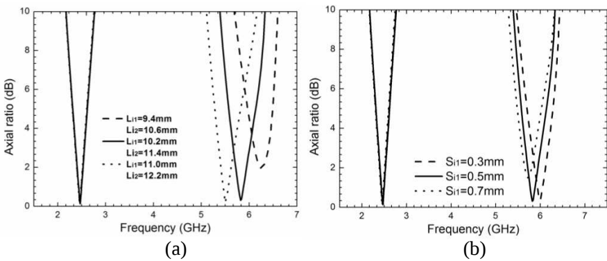
Figure 4. (a) Simulated axial ratio for different values of L_{i1} and L_{i2} . (b) Simulated axial ratio for different values of S_{i1} .
