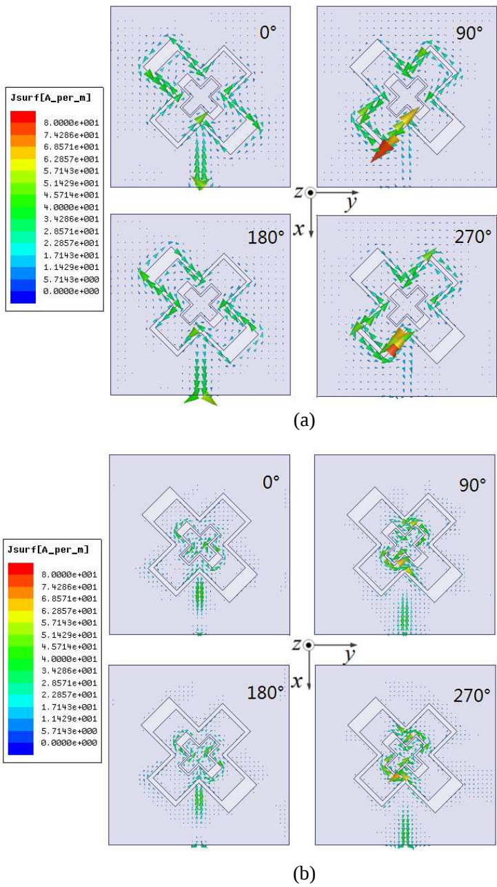
Figure 7. The simulated current distributions at the frequency of (a) 2.45 GHz (b) 5.8 GHz.
