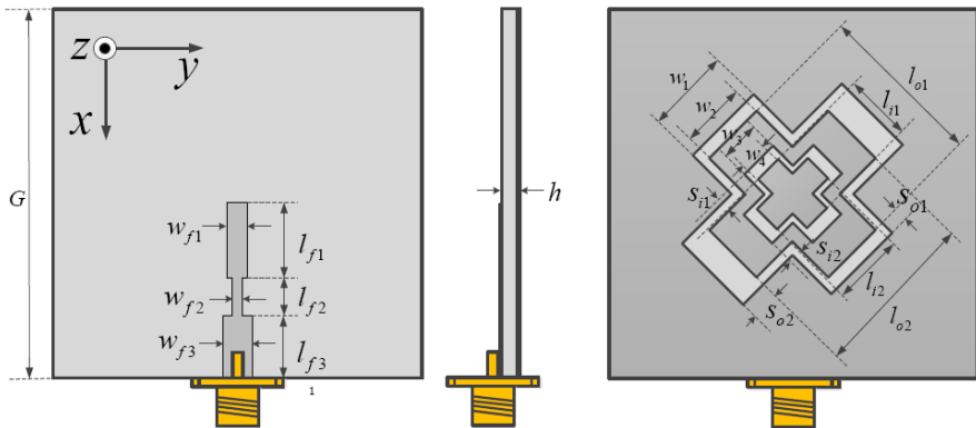
Figure 1. Configuration of the proposed antenna.
