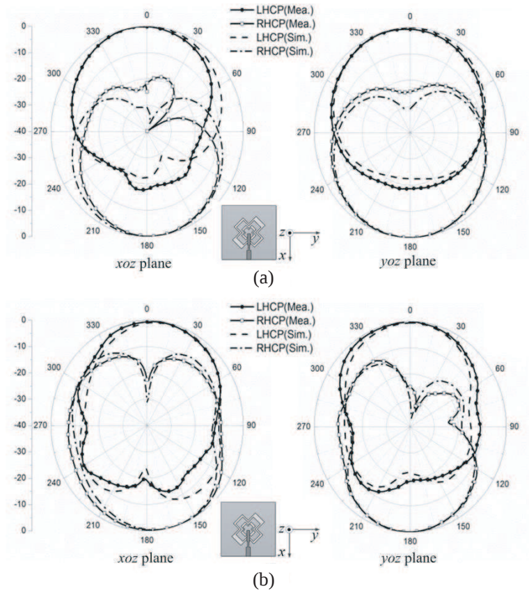
Figure 8. Simulated and measured radiation patterns at (a) 2.45 GHz, (b) 5.8 GHz.
