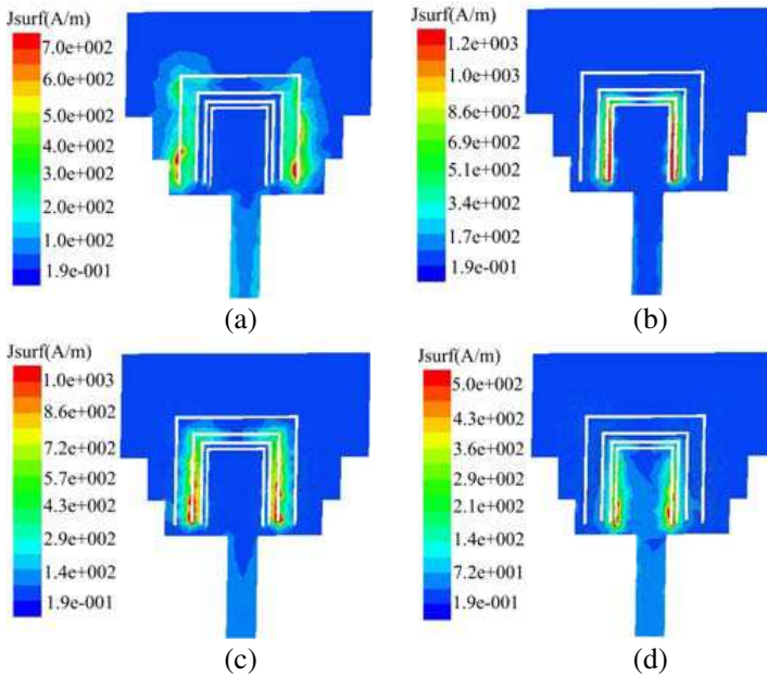
Figure 5. Current distribution on the conductors of the band-notched antenna at (a) 3.5 GHz, (b) 4.6 GHz, (c) 5.2 GHz and (d) 5.8 GHz.
