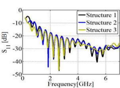
Figure 3. Return loss of three proposed structures.
