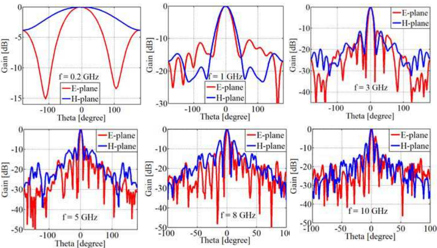
Figure 13. Simulated radiation patterns for array of elements with lens.
