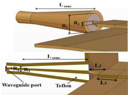
Figure 4. Transition between the coaxial cable and antenna.
