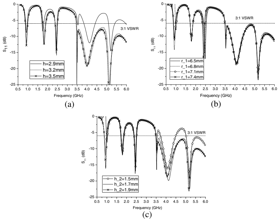
Figure 4. Simulated S_{11} of the proposed multiband antenna, (a) variations in h , (b) variations in r_1 , (c) variations in h_2 .
