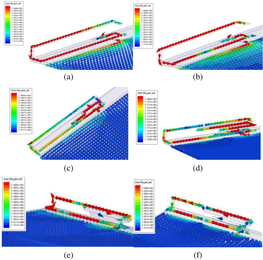
Figure 2. Surface currents on (a) IFA at 900 MHz, (b) IFA at 1.76 GHz, (c) IFA with a resonator at 2.45 GHz, (d) complete antenna at 3.5 GHz, (e) complete antenna at 5.2 GHz and (f) complete antenna at 5.8 GHz.
