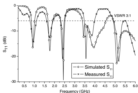
Figure 7. Measured and simulated S_{11} of the proposed antenna.
