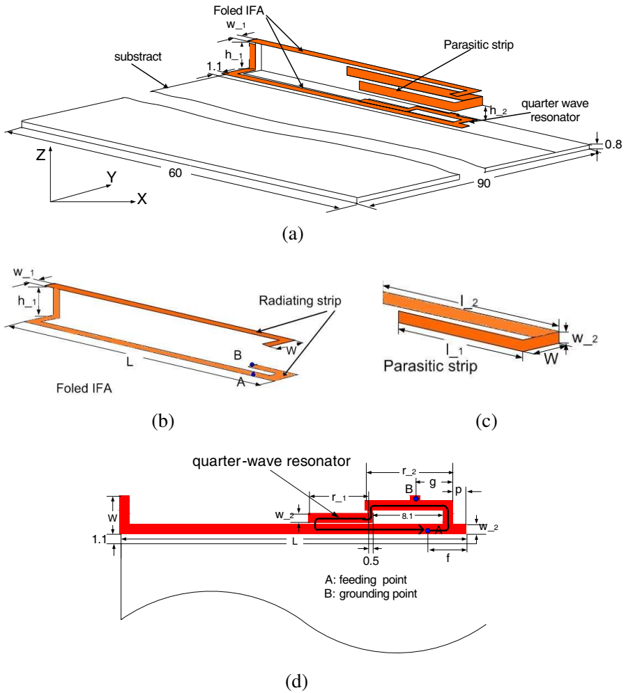
Figure 1. Geometry of the proposed antenna structures, (a) 3-D view, (b) folded IFA, (c) parasitic strip, (d) added resonator.
