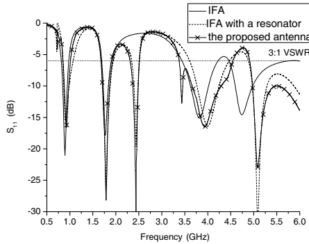
Figure 3. Simulated S_{11} of different antenna structures.
