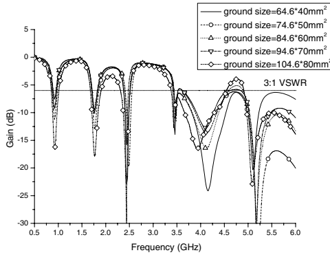
Figure 5. Simulated S_{11} of the proposed antenna variations in ground size.
