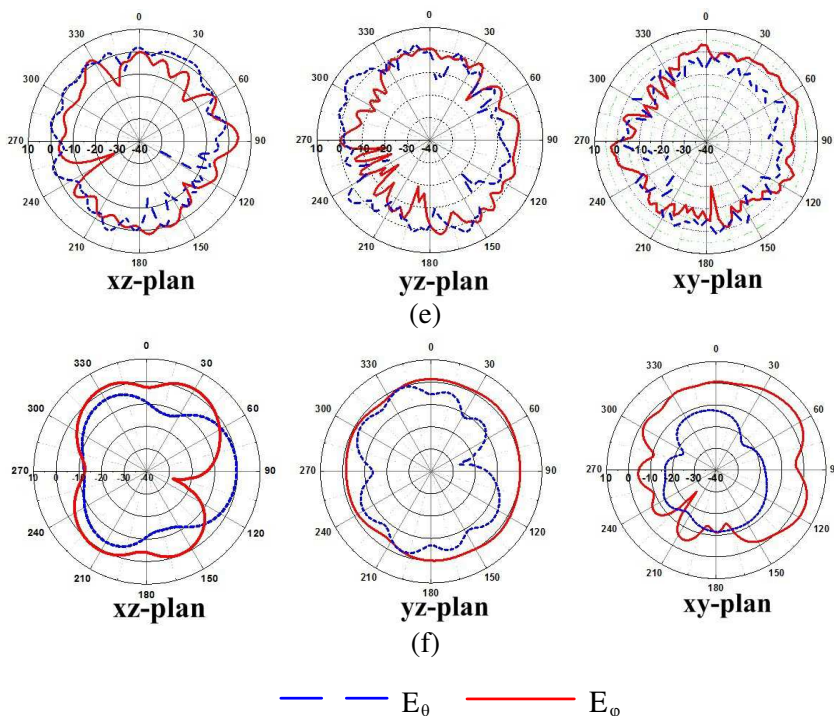
Figure 8. Radiation patterns (co-polarization and cross-polarization) of the proposed antenna at different frequencies (a) 0.9 GHz, (b) 1.76 GHz, (c) 2.45 GHz, (d) 3.5 GHz, (e) 5.2 GHz and (f) 5.8 GHz.
