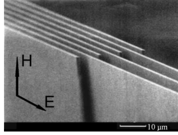
Figure 5. SEM image of a 1D PC with an inter-digital design. The number of periods, m = 6 , and the images shows the directions of the electric field vectors, for E - and H -polarization, of the incident light.
