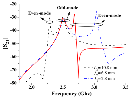
Figure 2. Resonant properties of the dual-mode slotline SISLR against L_3 .
