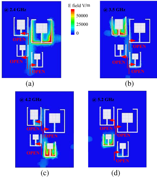
Figure 8. Electric field distributions for (a) the first channel @ 2.4 GHz. (b) The Second channel @ 3.5 GHz. (c) The third channel @ 4.2 GHz. (d) The fourth channel @ 5.2 GHz.
