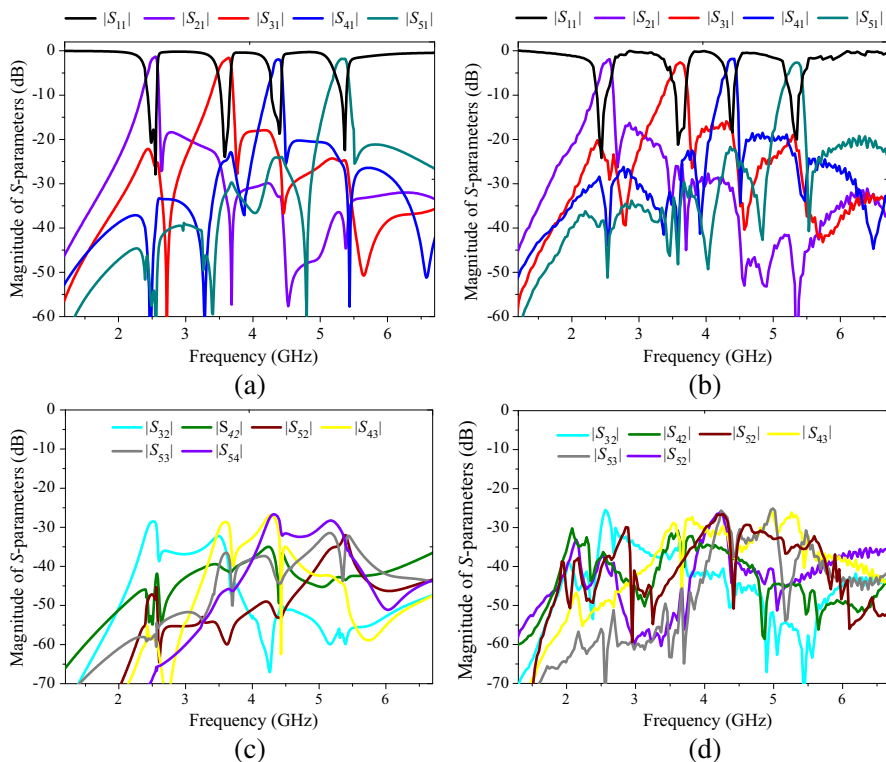
Figure 7. Response of the fabricated quadruplexer. (a) Simulated insertions and return losses. (b) Measured insertions and return losses. (c) Simulated isolation characteristic. (d) Measured isolation characteristic.
