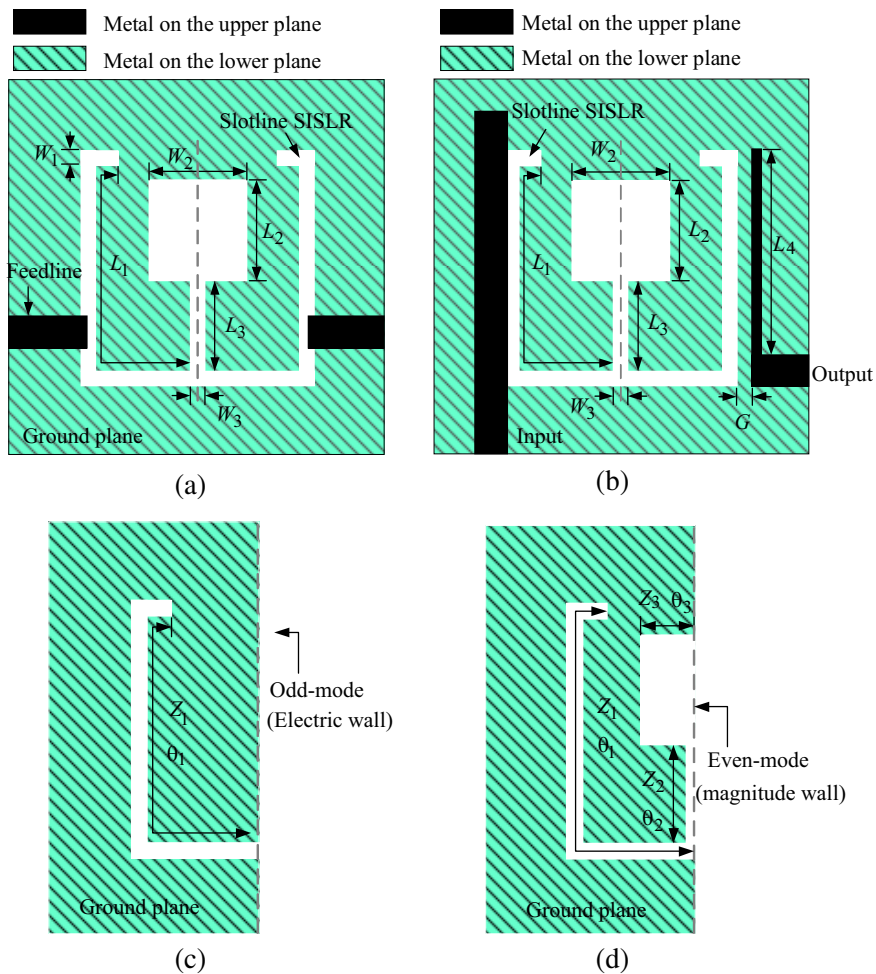
Figure 1. Circuit models for (a) dual-mode slotline SISLR. (b) Second-order slotline SISLR BPF. (c) Odd-mode for the slotline SISLR. (d) Even-mode for the slotline SISLR.
