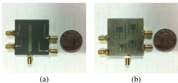
Figure 6. Photograph of the fabricated quadruplexer. (a) Top view. (b) Bottom view.
