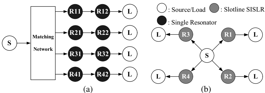
Figure 3. Coupling scheme of a quadruplexer with four two-order BPFs. (a) Conventional structure. (b) Proposed structure.
