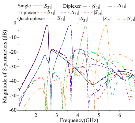
Figure 5. Simulated S parameters of a single-band BPF, diplexer, triplexer and quadruplexer.
