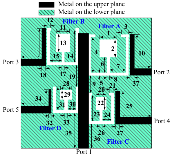
Figure 4. Layout of the proposed quadruplexer.
