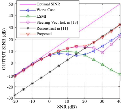
Figure 1. Output SINR versus SNR of the first example, T = 30 .
