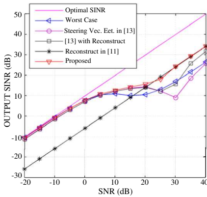
Figure 3. Output SINR versus SNR of the second example, T = 30 .
