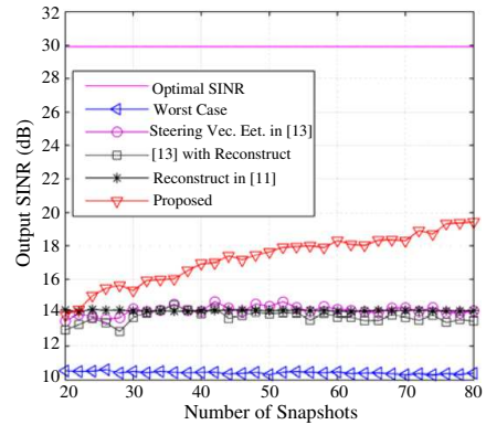
Figure 4. Output SINR versus the number of snapshots of the second example, \text{SNR} = 20 dB.
