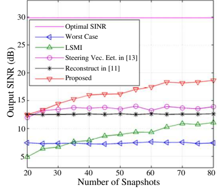
Figure 2. Output SINR versus the number of snapshots of the first example, SNR = 20 dB.
