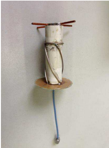
Figure 10. Photograph of the realized antenna.
