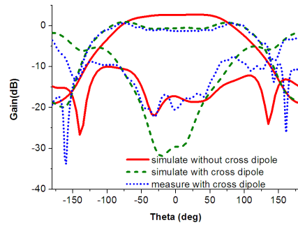
Figure 12. The simulated and measured CP gain patterns of the realized antenna along with the simulated result of the QHA without cross dipoles.
