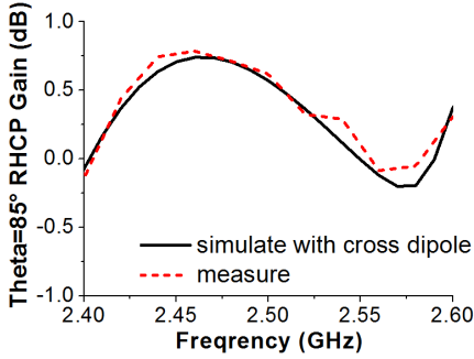
Figure 13. The simulated and measured results of the RHCP gain at 5° elevation angle versus frequency of the proposed antenna.
