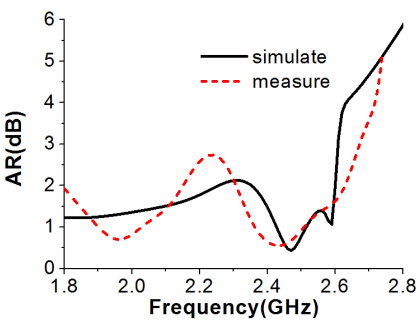
Figure 14. The simulated and measured results of the axial ratio at broadside versus frequency of the proposed antenna.
