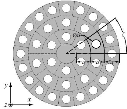
Figure 2. Top view of the GRIN metamaterial lens.
