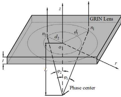
Figure 1. Geometry of the GRIN metamaterial lens.
