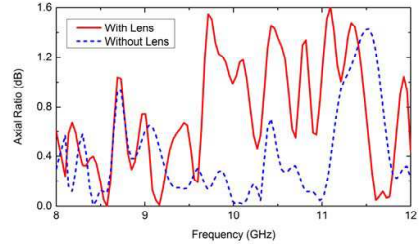
Figure 13. Measured axial ratio spectra of the circularly polarized horn antenna with and without GRIN metamaterial lens.
