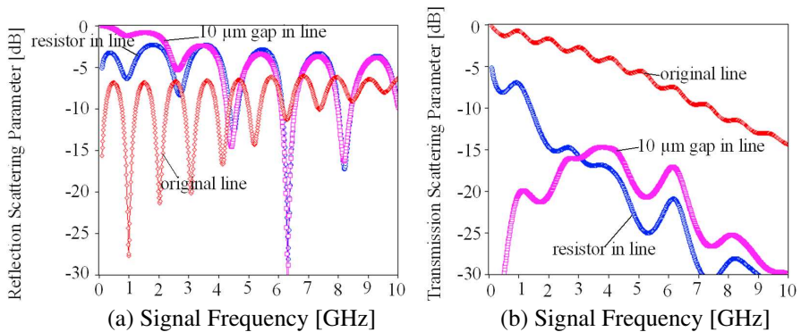
Figure 5. (a) Simulated reflection scattering response of the simulation model of the original CPW line with no discontinuity, with asymmetrical capacitive discontinuity, and with asymmetrical resistive discontinuity. (b) Simulated transmission scattering response of the simulation model of the CPW line with no discontinuity, with capacitive discontinuity, and with resistive discontinuity.
