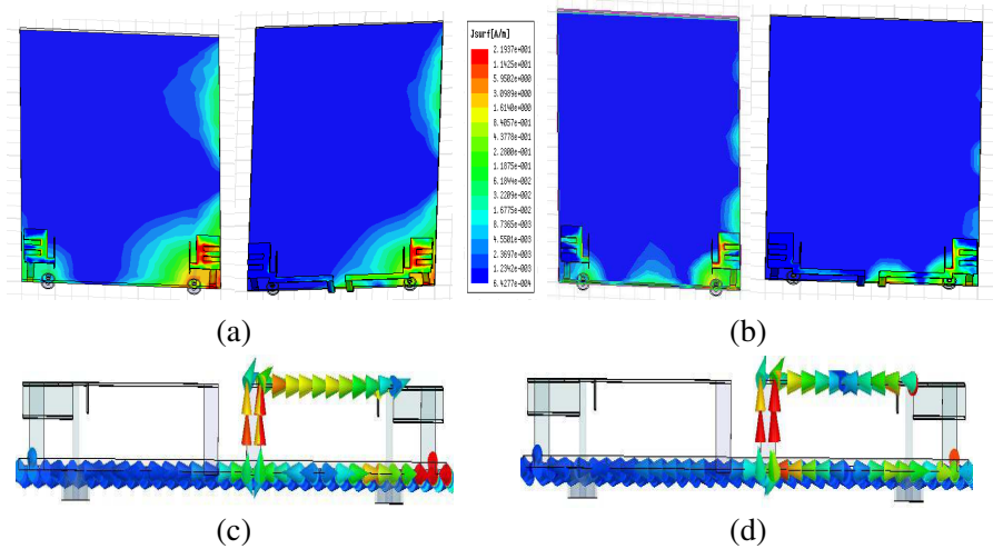
Figure 6. (a) Surface current distribution at 2.45 GHz. (b) Surface current distribution at 5.5 GHz. (c) Surface current flow vector on folded shoring strip at 2.45 GHz. (d) Surface current flow vector on folded shoring strip at 5.5 GHz.
