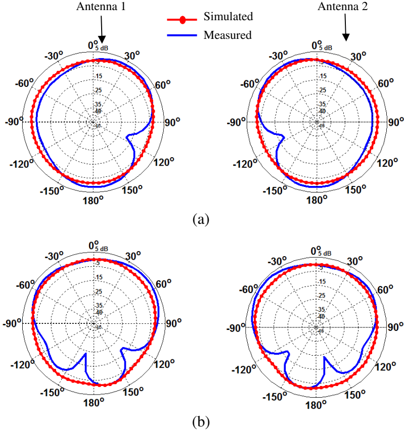
Figure 7. Measured radiation pattern of proposed structure in YZ plane (a) at 2.45 GHz (b) at 5.5 GHz.
