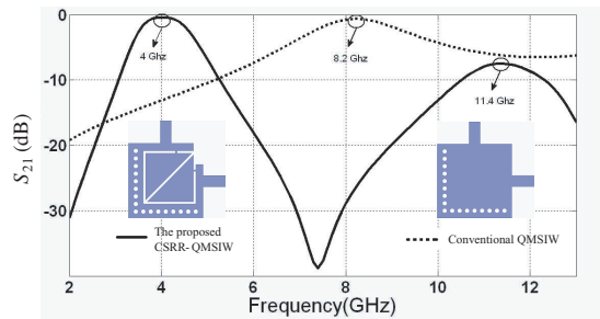
Figure 7. Full-wave simulated S_{21} of conventional QMSIW and the proposed CSRR-QMSIW.
