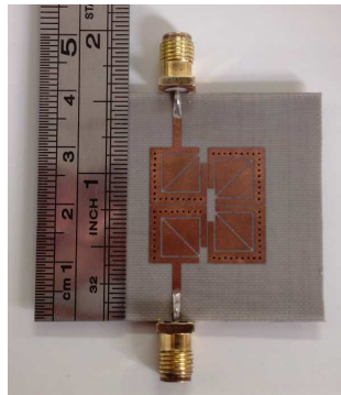
Figure 13. Photograph of fabricated BPF.
