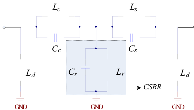
Figure 8. Equivalent lumped circuit of the proposed CSRR-QMSIW resonator.
