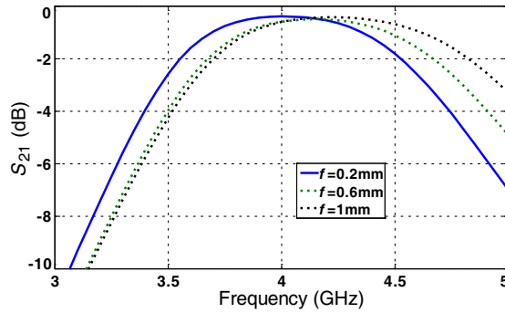
Figure 3. Simulated S_{21} of CSRR-QMSIW resonator with f = 0.2 mm, f = 0.6 mm, f = 1 mm.
