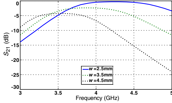
Figure 5. Simulated S_{21} of CSRR-QMSIW resonator with w = 2.5 mm, w = 3.5 mm, w = 4.5 mm.
