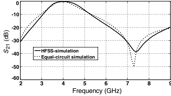
Figure 9. Transmission responses by equivalent circuit model and full-wave simulation.
