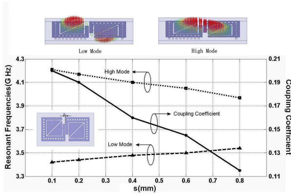
Figure 11. Vector electric field distribution, resonance frequencies of the two excited modes and the calculated coupling coefficient versus the distance s .
