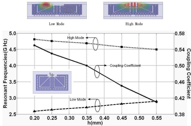
Figure 12. Vector electric field distribution, resonance frequencies of the two excited modes and the calculated coupling coefficient versus the distance h .
