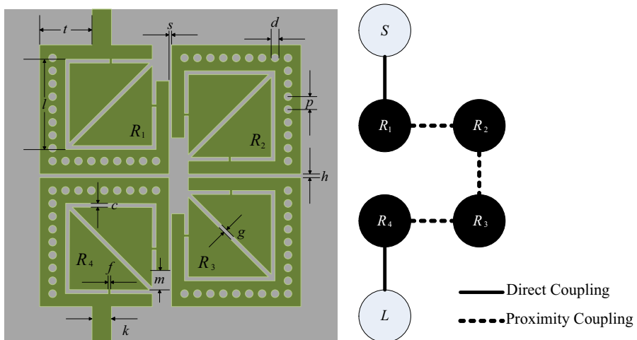
Figure 10. The proposed CQ filter and its general coupling structure.
