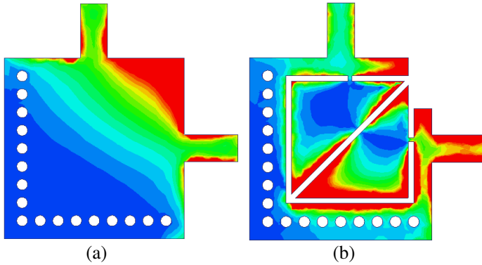
Figure 2. Surface current distribution. (a) Conventional QMSIW, (b) the proposed CSRR loaded QMSIW.
