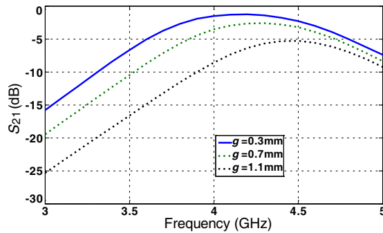
Figure 4. Simulated S_{21} of CSRR-QMSIW resonator with g = 0.3 mm, g = 0.7 mm, g = 1.1 mm.
