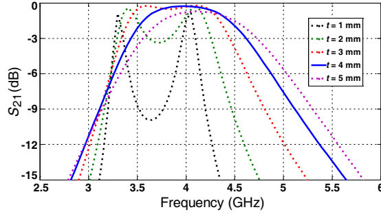
Figure 6. Simulated S_{21} of CSRR-QMSIW resonator with t = 1 mm, t = 2 mm, t = 3 mm, t = 4 mm, t = 5 mm.
