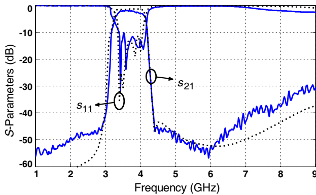
Figure 14. Measured and simulated results of the proposed BPF.
