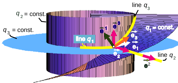
Figure 3. Coordinate surfaces and coordinate lines of curvilinear coordinates system (q_1, q_2, q_3) , defined as q_1 = z/\theta ; q_2 = \varrho ; q_3 = z , where cylindrical coordinates \varrho, \theta and z are used. In this case, coordinate plane q_3 = \text{constant} describes the wave-front and coordinate line q_3 is along the desired ray.
