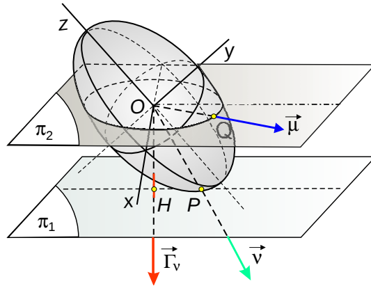
Figure 1. Cauchy's quadric associated with a second-order tensor \tilde{I} . The orthogonality of vectors \bar{\Gamma}_\nu = \tilde{I} \cdot \hat{\nu} and \hat{\mu} implies that unit vectors \hat{\nu} and \hat{\mu} are conjugate directions. Vector \hat{\mu} lies in plane \pi_2 parallel to the tangent plane of the ellipsoid at "P".
