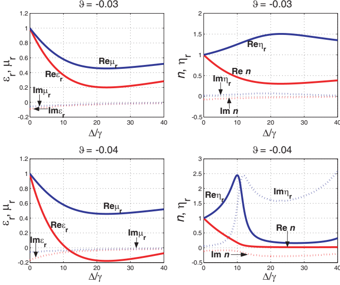
Figure 5. The dispersion characteristics of the relative permittivity \epsilon_r , the relative permeability \mu_r , the relative impedance \eta_r and the refractive index n of the atomic vapor when the incident probe field becomes strong. The electric Rabi frequency of the incident probe field is chosen as \Omega_E = 3.0 \times 10^7 \text{ s}^{-1} .
