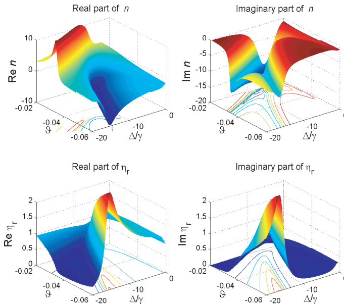
Figure 3. The tunable behavior of dispersion of the real and imaginary parts of the refractive index n and the relative impedance \eta_r .
