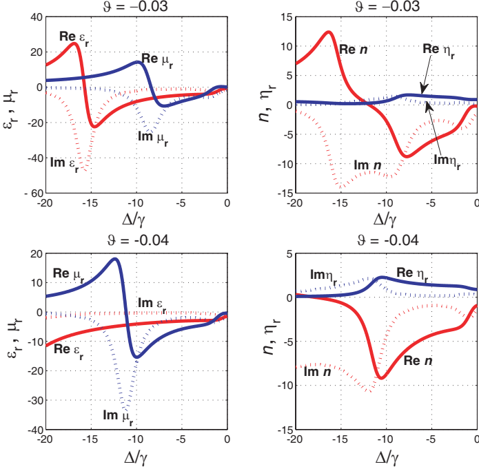
Figure 2. The dispersion characteristics of the relative permittivity \epsilon_r , the relative permeability \mu_r , the relative impedance \eta_r and the refractive index n of the atomic vapor driven by the incoherent pump field (for high-gain amplification) and the strong coupling field (for generating dressed states). The electric Rabi frequency of the incident probe field is chosen as \Omega_E = 5.0 \times 10^6 \text{ s}^{-1} .
