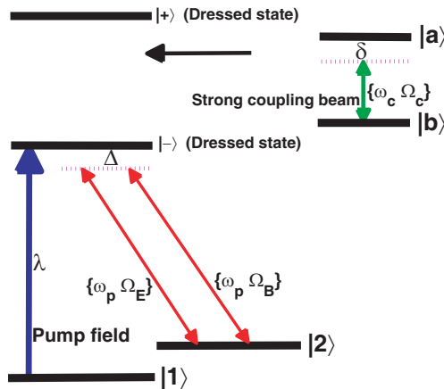
Figure 1. The schematic diagram for the pumped dressed-state mixed-parity transitions. The electric-dipole allowed transition |a\rangle - |b\rangle is driven by a strong coupling laser beam, and two dressed states |+\rangle and |-\rangle will result from the linear combinations of the two bare levels |a\rangle and |b\rangle . The energy level pair |2\rangle - |-\rangle is coupled to the electric and magnetic fields of a probe beam whose electric and magnetic Rabi frequencies are \Omega_E and \Omega_B , respectively. Both electric- and magnetic-dipole allowed transitions (between the bare level |2\rangle and the mixed-parity dressed level |-\rangle ) will occur, and hence simultaneously negative permittivity and permeability would be achieved through the pumped dressed-state transitions.
