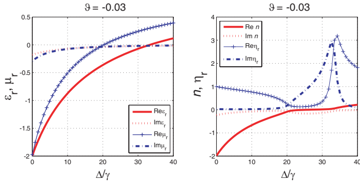
Figure 6. The dispersion characteristics of the relative permittivity \varepsilon_r , the relative permeability \mu_r , the relative impedance \eta_r and the refractive index n of the atomic vapor when the incident probe field is weak, i.e., the electric Rabi frequency of the incident probe field is chosen as \Omega_E = 5.0 \times 10^2 \text{ s}^{-1} .
