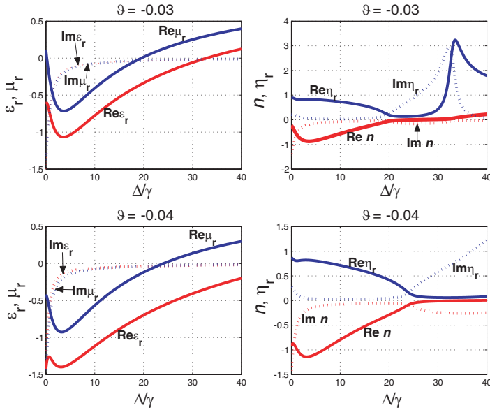
Figure 4. The dispersion characteristics of the relative permittivity \epsilon_r , the relative permeability \mu_r , the relative impedance \eta_r and the refractive index n of the atomic vapor with incoherent gain. All the atomic and optical parameters are chosen exactly the same as those in Fig. 2.
