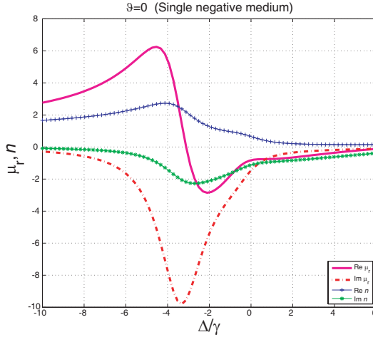
Figure 7. The real and imaginary parts of the relative permeability \mu_r and the refractive index n when the strong coupling field is switched off (i.e., the Rabi frequency \Omega_c = 0 and hence the dressed-state mixing angle \vartheta = 0 ).
