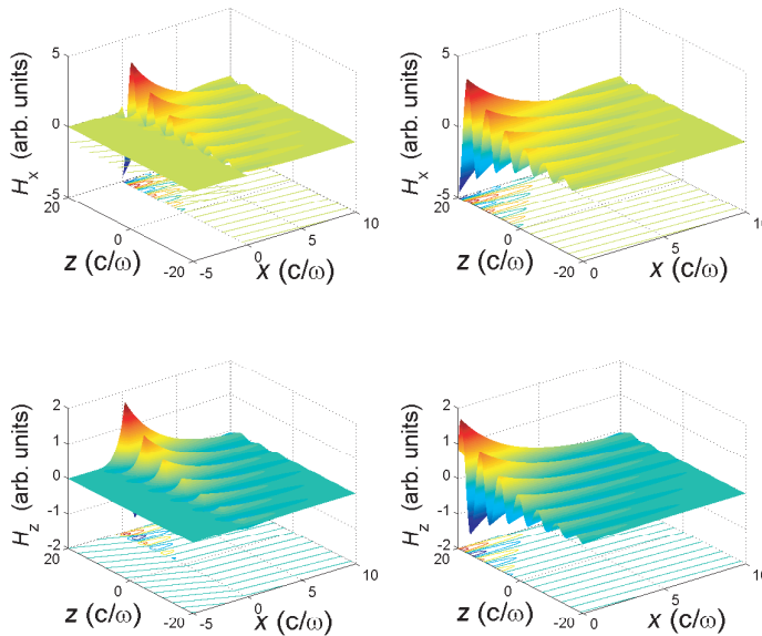
Figure 8. The spatial field profile of a TE-mode surface plasmon wave at the interface between the dielectric of \mu_r = 1 and the single negative atomic medium. The negative-permeability atomic medium is in the half space x < 0 and the dielectric in the other half space x > 0 .
