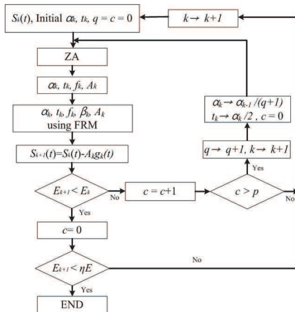
Figure 5. Proposed method for chirplet decomposition.
