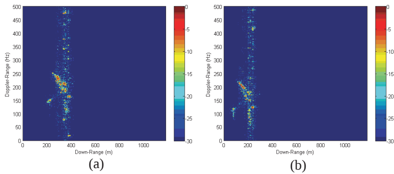
Figure 6. Two ISAR image of Boeing 747. (a) Image 1 (300~573th pulses). (b) Image 2 (2500~2773th pulses).
