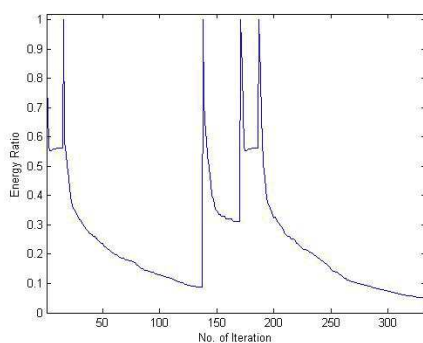
Figure 7. Convergence curve of Fig. 6(a).
