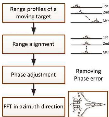
Figure 1. Procedure of RDA.
