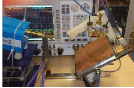
Figure 7. Measurement system with the metallic sheet. Both horns are placed at 50^\circ of elevation in specular direction.
