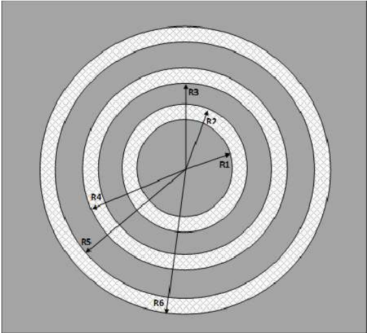
Figure 4. Layout of the Fresnel reflector.
