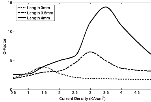
Figure 10. Variation of Q -factor with current densities for three different QD-SOAs length, when the other parameters are kept fixed.
