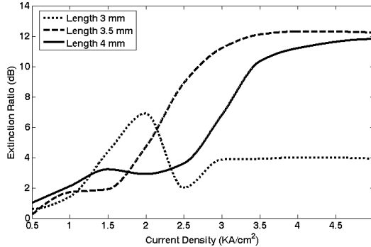
Figure 6. Variation of ER with current densities for three different QD-SOAs length, keeping other parameters fixed.
