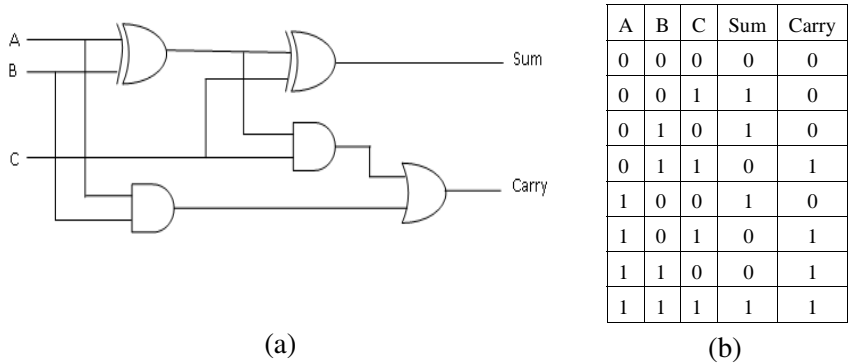
Figure 2. (a) Full adder logic diagram and (b) its truth table.
