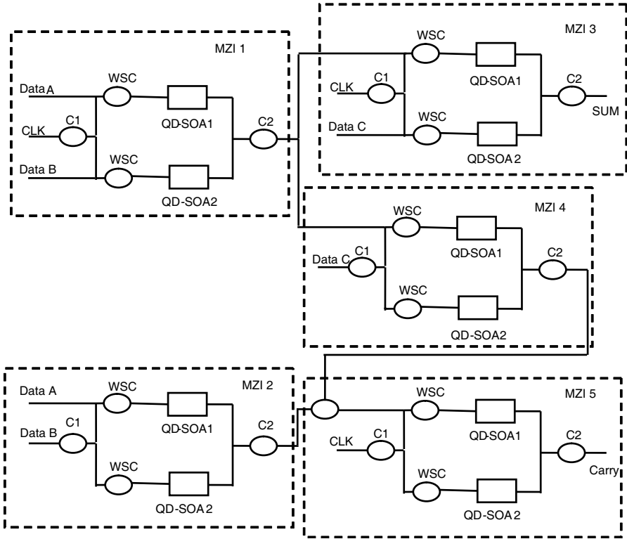
Figure 3. Configuration of the proposed all-optical full adder using five symmetrical QD-SOAs based MZI interferometers.
