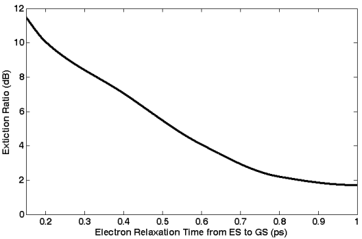
Figure 8. Variation of ER with electron relaxation time from the ES to the GS.
