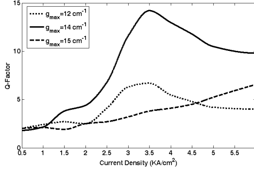
Figure 9. Variation of Q -factor with current densities for three different maximum modal gains, when the other parameters are kept constant.
