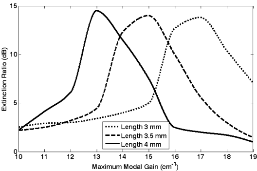
Figure 7. Variation of ER with the maximum modal gain for three different QD-SOAs length, keeping other parameters fixed.
