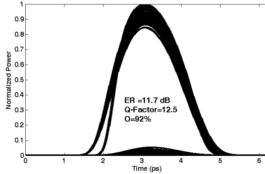
Figure 12. Simulated output waveforms with pseudo-eye-diagram (PED).
