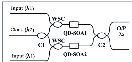
Figure 1. Schematic diagram of the all-optical QD-SOA-based MZI switch. WSC: wavelength-selective coupler; C1 and C2: Couplers.
