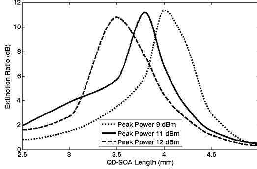
Figure 5. Variation of extinction ratio (ER) with QD-SOA length for different peak data power, keeping other parameters fixed.
