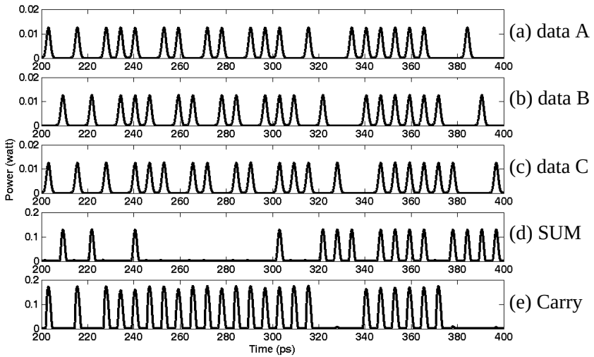
Figure 11. Waveforms of all-optical full adder, where (a) input data stream A, (b) input data stream B, (c) input data stream C ( C_{in} ), (d) output sum-bit (S) and (e) output carry-bit ( C_{out} ).
