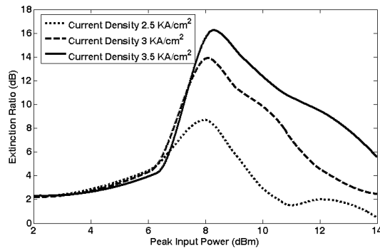
Figure 4. Variation of extinction ratio (ER) with peak data power for different current densities, keeping other parameters fixed.
