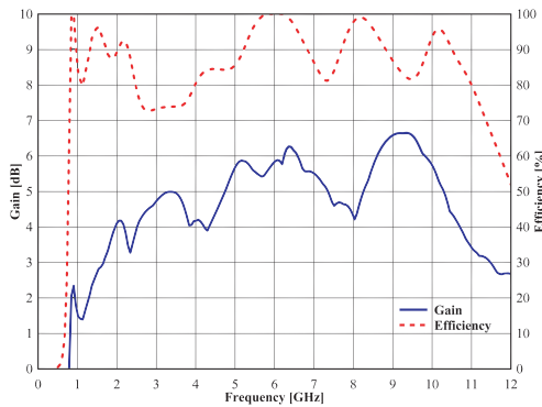
Figure 6. Simulated maximum gain and total efficiency.
