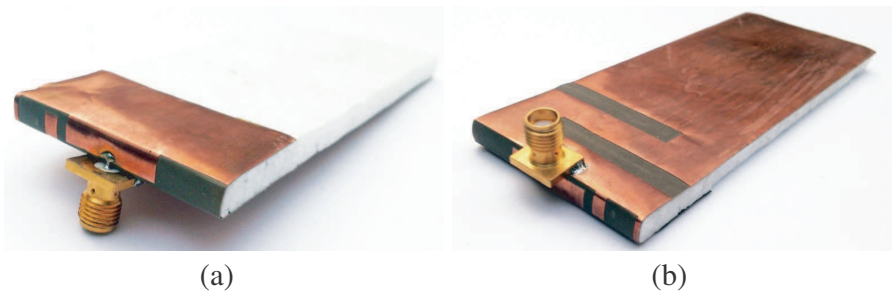
Figure 3. Pictures of the prototype. (a) Front view. (b) Back view.
