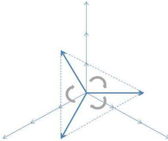
Figure 1. A schematic showing the symmetric tetrahedron formed by the permutation of the coordinates of either the electric or the magnetic field components. Their common summand must then lie on the height of the tetrahedron drawn from the origin of the coordinate system.
