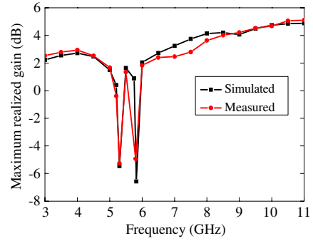
Figure 9. Simulated and measured maximum realized gain.
