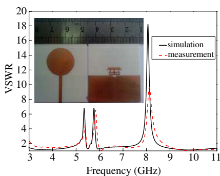
Figure 10. Comparison of the measured and simulated VSWR values of the tri-band notched UWB antenna.
