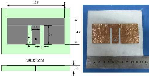
Figure 1. Geometry of planar E-shaped textile antenna.
