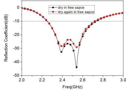
Figure 11. Comparison of the reflection coefficients of antenna in dry and dry-again states.
