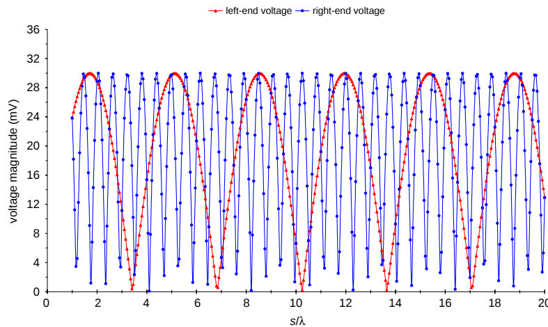
Figure 2. Plot of the left-end load voltage |V_0| and the right-end voltage |V_L| as functions of s/\lambda for a plane-wave excited straight-wire line with b/\lambda = 0.03 . The line is terminated in matched loads ( Z_0 = Z_L = Z_c ) and the angle of incidence is \theta_0 = 3\pi/4 .
