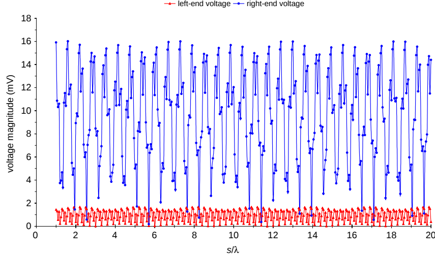
Figure 3. Like Fig. 2, but for a twisted-wire line with b/\lambda = 0.03 and p/\lambda = 0.3 .
