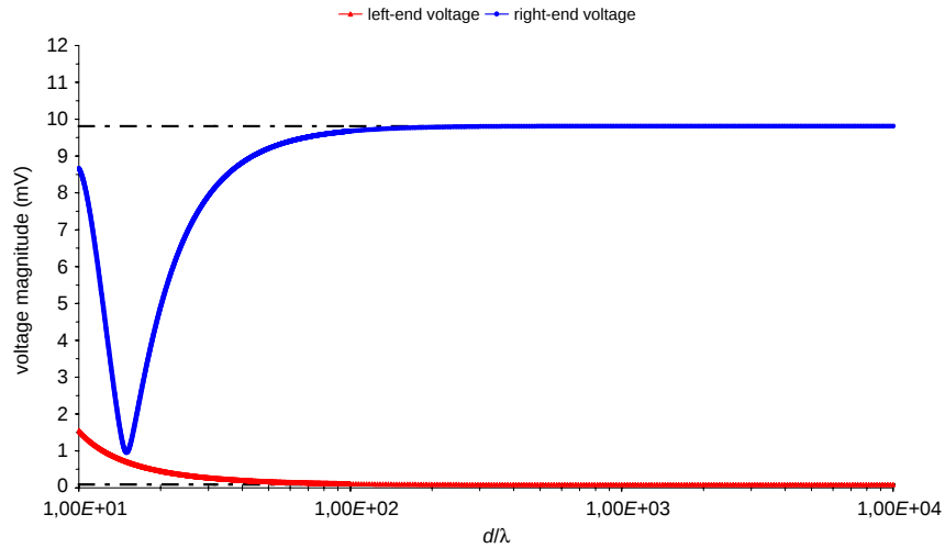
Figure 5. Like Fig. 4, but for the excitation field of (14)–(16) with x_0 = d , z_0 = d + s/2 , h/\lambda = w/\lambda = 0.337 and B given by (20).
