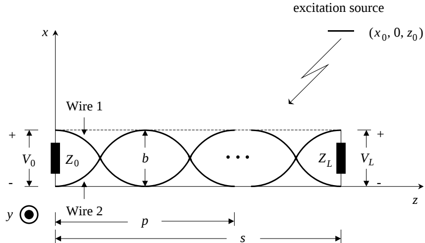
Figure 1. Sketch of a terminated twisted-wire pair, together a convenient coordinates system.
