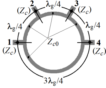
Figure 1. The conventional 3-dB ring coupler [1].
