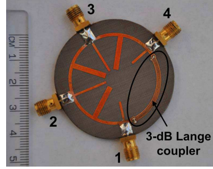
Figure 5. Photo of the fabricated broadband and small-size fully distributed CRLH based 3-dB ring coupler.
