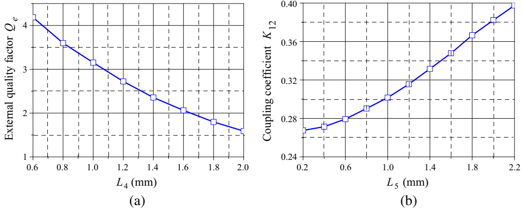
Figure 4. Design curves for (a) external quality factor Q_e and (b) coupling coefficients K_{12} .
