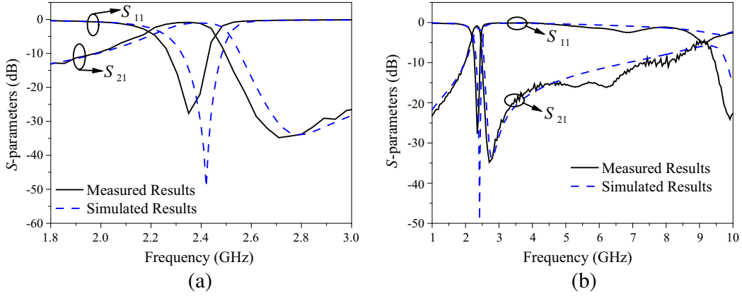
Figure 5. Simulated and measured results of the second-order filter. (a) Insertion loss and return loss, (b) wide-band response.
