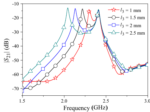
Figure 2. Simulated S_{21} -magnitude of the inductive-coupled quarter-wavelength resonators with different l_3 under weak coupling.
