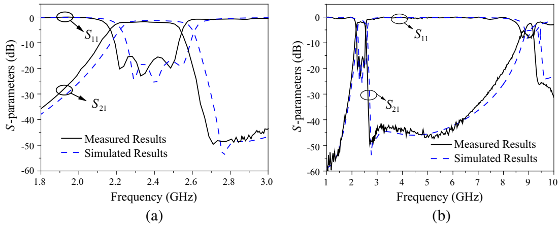
Figure 7. Simulated and measured results of the forth-order filter. (a) Insertion loss and return loss, (b) wide-band response.
