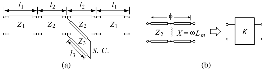
Figure 1. (a) Schematic of the inductive-coupled quarter-wavelength stepped-impedance resonators, (b) equivalent circuit model of the K -inverter.
