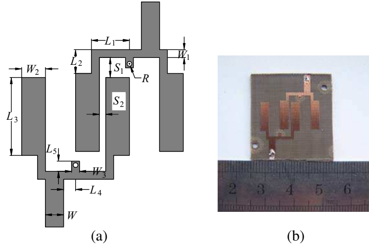
Figure 6. Configuration and photograph of the proposed forth-order filter. (a) Configuration, (b) photograph.
