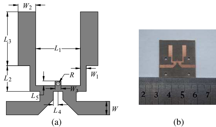
Figure 3. Configuration and photograph of the proposed second-order filter. (a) Configuration, (b) photograph.
