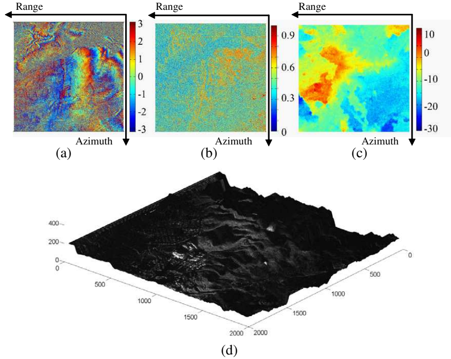
Figure 12. The BiInSAR result. (a) Interferometric phase after interferogram flattening and filtering. (b) Correction coefficient. (c) Unwrapped phase. (d) DEM.
