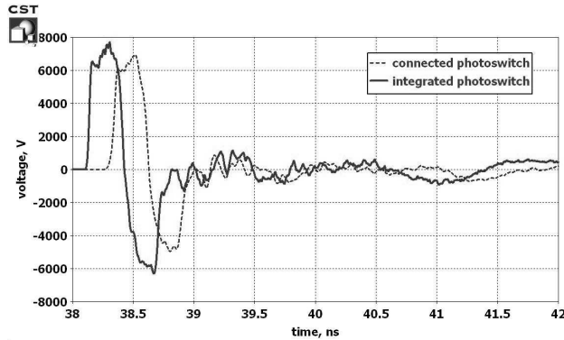
Figure 13. Voltage waveform at the antenna input.
