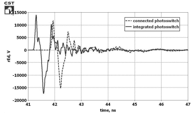
Figure 14. Waveforms of radiated electric fields.
