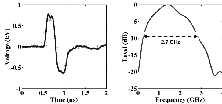
Figure 3. Bipolar pulse of 650 ps and its normalized spectrum.
