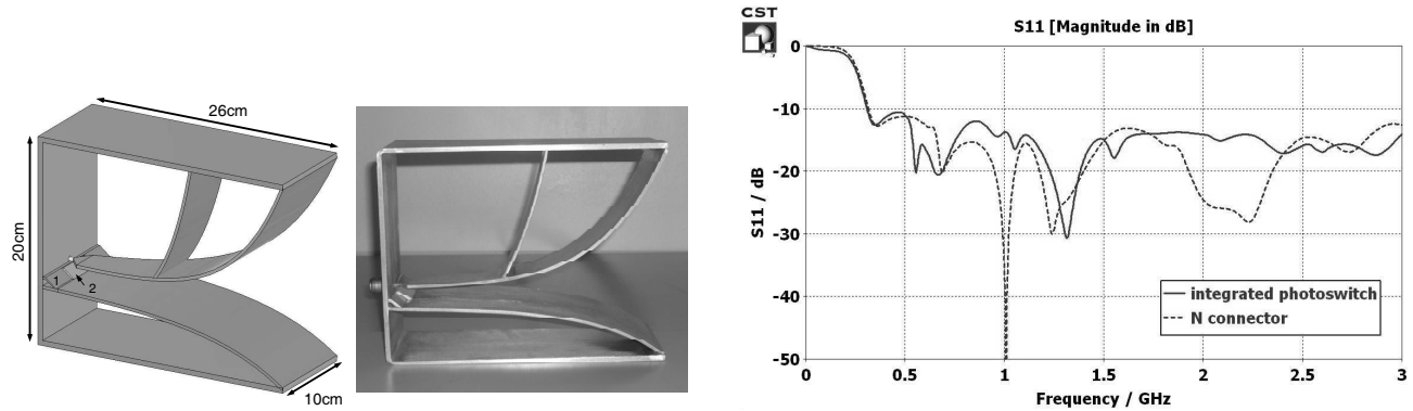
Figure 8. The UWB antenna (CAD model and realized geometry).
