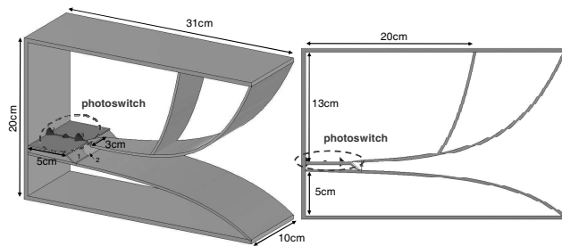
Figure 10. Views of the antenna with integrated photoconductor device.
