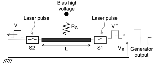
Figure 2. Bipolar frozen-wave generator principle.
