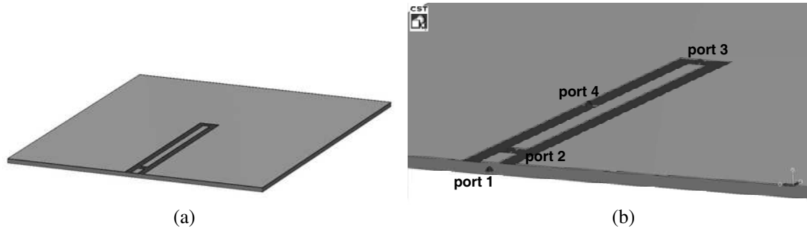
Figure 4. 3D view of coplanar waveguide for EM simulation with CST MWS. (a) General view. (b) Zoom on coplanar waveguide with port location.
