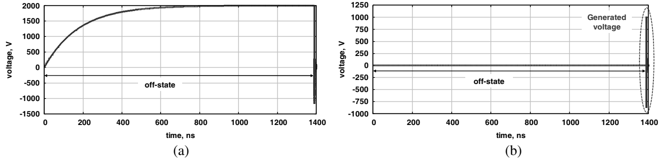
Figure 6. Charging voltage of (a) the coplanar waveguide and (b) generated voltage.
