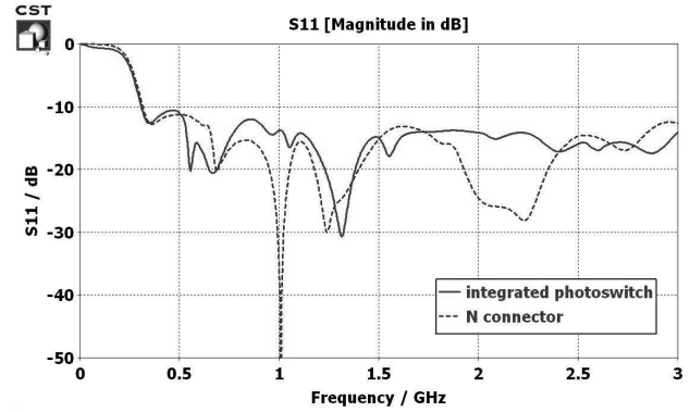
Figure 9. Reflection coefficient.
