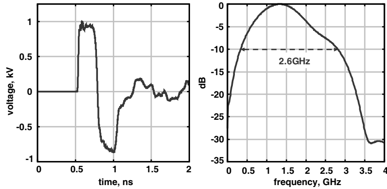
Figure 7. Theoretical bipolar pulse and its normalized spectrum.
