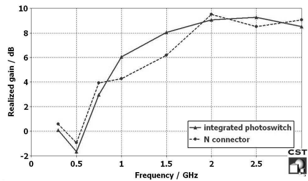
Figure 11. Realized gain in the main radiation direction.
