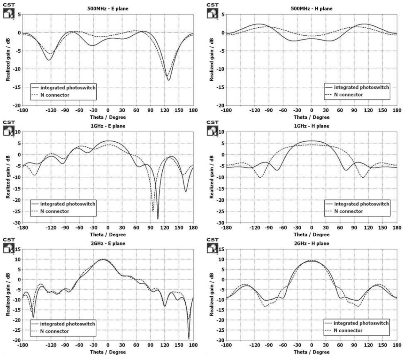
Figure 12. Radiation patterns for E and H planes.
