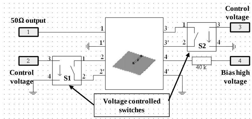
Figure 5. Circuit model of the photoswitch.
