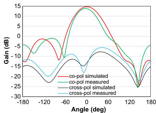
Figure 5. Simulated and measured E -plane radiation pattern of antenna array.
