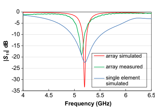
Figure 3. Simulated and measured return loss of proposed antenna.
