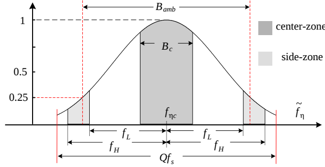
Figure 2. Illustration of the PSD of the rightly reconstructed azimuth signal (square of the round-trip azimuth antenna pattern).
