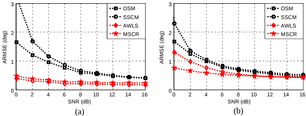
Figure 4. ARMSE of the phase error estimates versus SNR in the cases of (a) uniform sampling, \text{PRF} = 125 Hz; (b) nonuniform sampling, \text{PRF} = 142.86 Hz.
