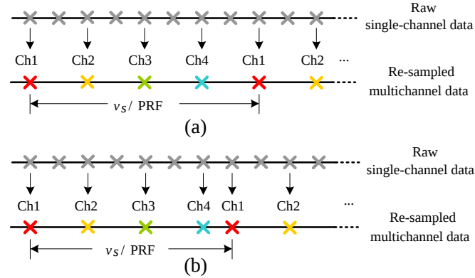
Figure 3. Azimuth positions of the raw single channel data and the synthesized multichannel data. (a) Uniform sampling, \text{PRF} = 125 Hz. (b) Nonuniform sampling, \text{PRF} = 142.86 Hz.
