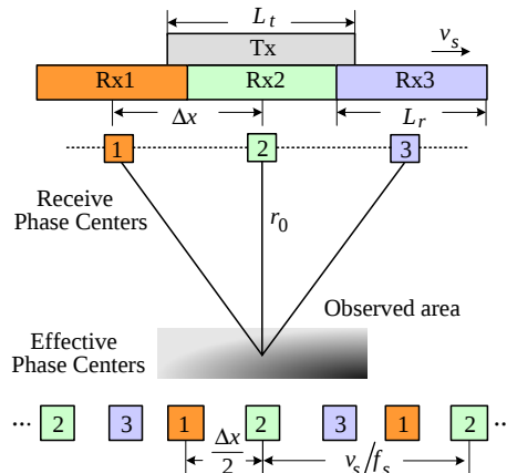
Figure 1. Spatial sampling of azimuth multichannel SAR.
