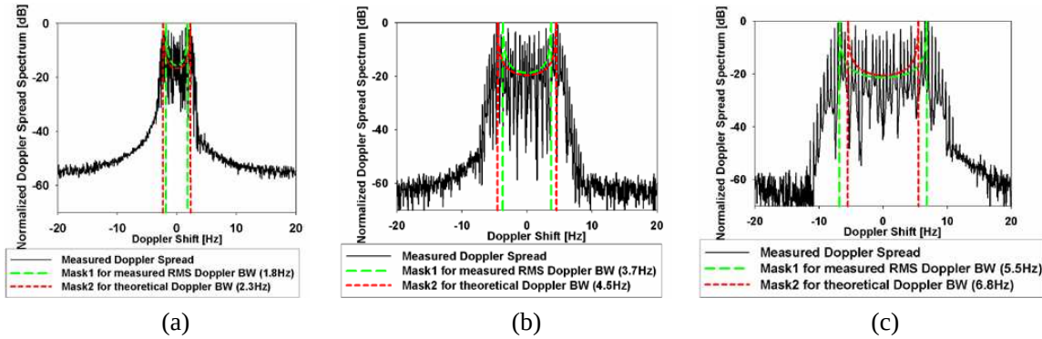
Figure 3. The measured Doppler spread spectrum with platform stirring in the AC. (a) Platform at 10 RPM in CW. (b) Platform at 20 RPM in CW. (c) Platform at 30 RPM in CW.
