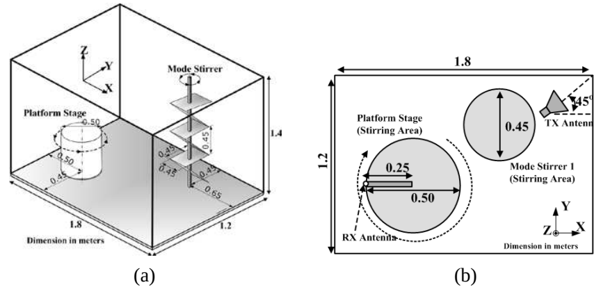
Figure 2. The measurement setup of the RC. (a) The geometries of the RC. (b) The configuration of TX and RX antennas in the RC.
