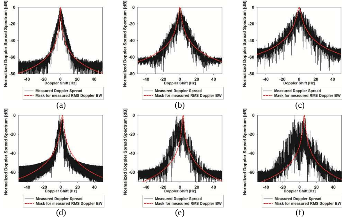
Figure 4. The measured Doppler spread spectrum with either Mode or Platform stirring in the RC. (a) Mode stirrer at 3 RPM in CW. (b) Mode stirrer at 6 RPM in CW. (c) Mode stirrer at 9 RPM in CW. (d) Platform at 10 RPM in CW. (e) Platform at 20 RPM in CW. (f) Platform at 30 RPM in CW.
