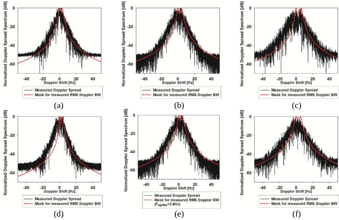
Figure 5. The measured Doppler spread spectrum with either Mode or Platform stirring in the RC. (a) Platform at 10 RPM in CW and Mode stirrer at 6 RPM in CW. (b) Platform at 20 RPM in CW and Mode stirrer at 6 RPM in CW. (c) Platform at 30 RPM in CW and Mode stirrer at 6 RPM in CW. (d) Platform at 20 RPM in CW and Mode stirrer at 3 RPM in CW. (e) Platform at 20 RPM in CW and Mode stirrer at 6 RPM in CW. (f) Platform at 20 RPM in CW and Mode stirrer at 9 RPM in CW.
