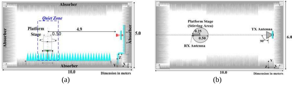
Figure 1. The measurement setup of the AC. (a) The geometries of the AC. (b) The configuration of TX and RX antennas in the AC.
