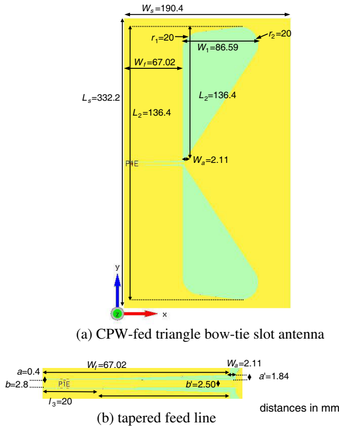
Figure 1. (a) Geometry of the triangle bowtie slot antenna modeled using FDTD simulations; (b) Top view of the tapered feed line (distances in mm).
