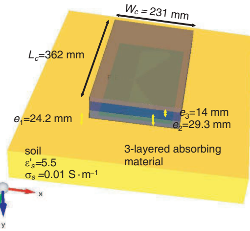
Figure 3. Geometry of the shielded slot bowtie modeled using FDTD simulations.
