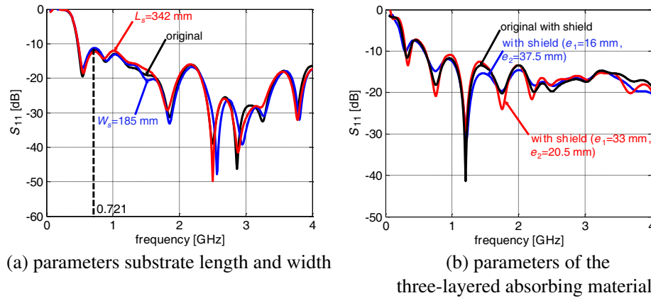
Figure 5. Influence of antenna geometrical parameters on the return loss S_{11\text{dB}}(f) ; (a) Substrate length and width; (b) The three-layered absorbing material.
