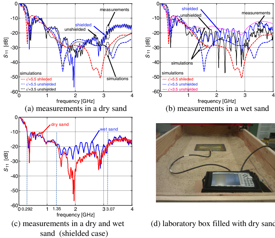
Figure 8. Comparison of theoretical and experimental return losses S_{11\text{dB}}(f) ; (a) In a dry and (b) a wet soil; (c) Comparison of measurement results only in a dry and a wet soil; (d) Experimental setup on a dry sand.
