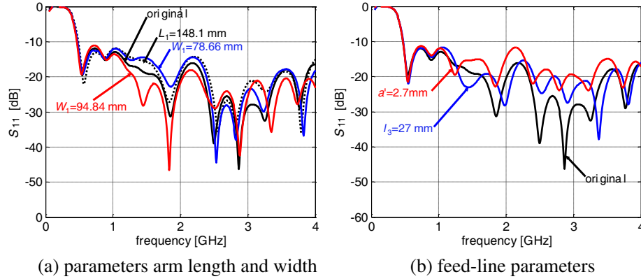
Figure 4. Influence of antenna geometrical parameters on the return loss S_{11\text{dB}}(f) ; (a) Arm length and width; (b) Feed-line.
