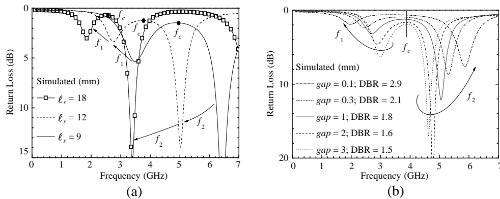
Figure 8. The dual-band mechanism. (a) Central-stop frequency shifting and (b) dual-band ratio.
