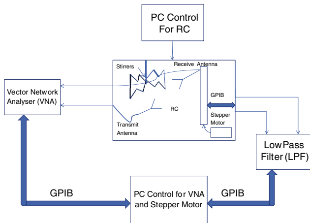
Figure 1. Block-diagram showing measurement setup for propagation measurements in RC.
