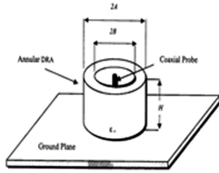
Figure 11. Probe fed annular DRA.
