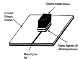
Figure 8. Multisegment DRA.
