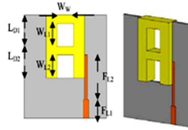
Figure 20. A-shaped DRA mounted on a vertical ground plane edge [101].
