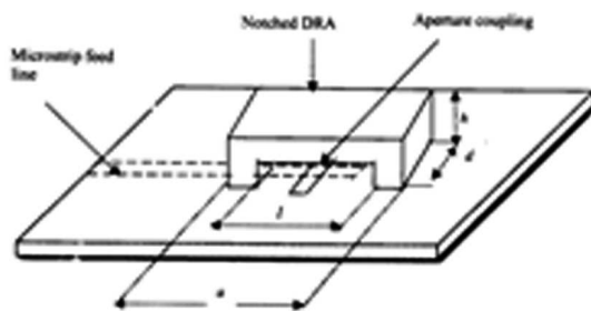
Figure 1. Notched rectangular DRA with aperture slot coupling [6].
