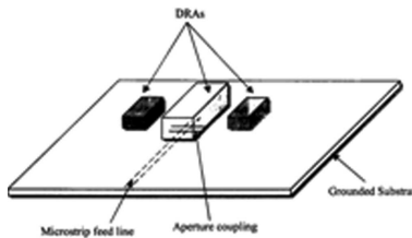
Figure 13. Slot fed rectangular DRA with two parasitic elements [75].
