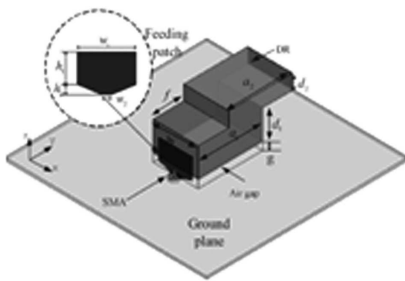
Figure 17. Geometry of Z-shaped UWB DRA [96].
