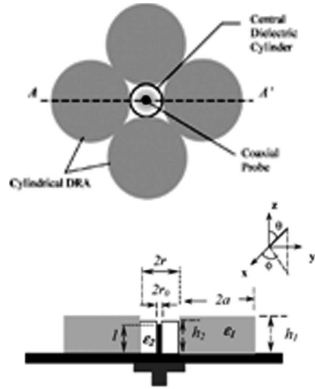
Figure 9. Four elements cylindrical DRA fed by a central coaxial probe [51].
