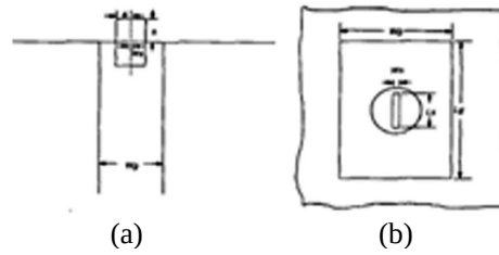
Figure 23. Configuration of waveguide excited DRA (a) side view, (b) top view [121].
