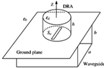
Figure 5. Geometry of the DRA excited by a narrow slot in a rectangular waveguide [34].
