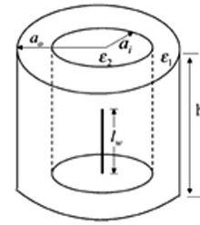
Figure 12. Proposed stacked double annular-ring DRA [72].
