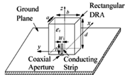
Figure 2. Configuration of strip-fed rectangular DRA [15].
