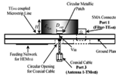
Figure 22. Side view of the triple mode DRA [116].
