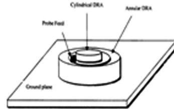
Figure 14. Probe-fed annular DRA with embedded parasitic cylindrical DRA [75].
