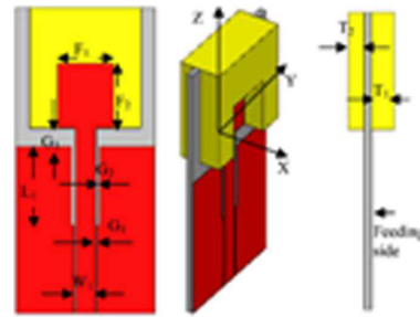
Figure 18. Geometry of the proposed inserted UWB DRA excited by CPW feeding [97].
