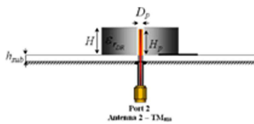
Figure 21. Dual-band DRA [113].
