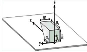
Figure 3. Probe fed trapezoidal DRA [31].
