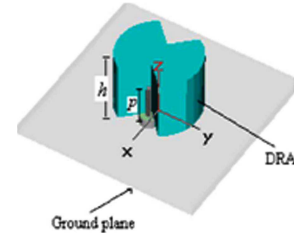
Figure 4. Broadband bowtie DRA [33].
