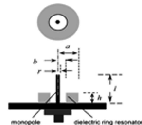
Figure 16. Top and cross-sectional views of a monopole-DRA proposed in [88].
