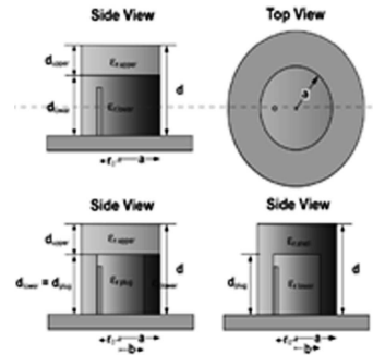
Figure 10. Stacked and embedded cylindrical DRA [52].
