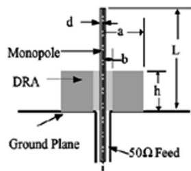
Figure 15. Cross section of the hybrid monopole-DRA [79].
