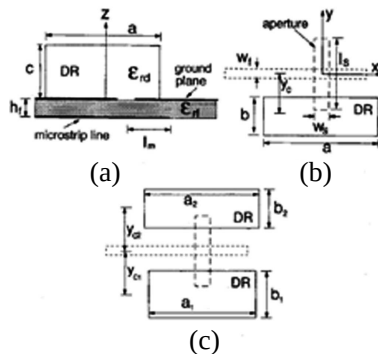
Figure 7. (a) Side and (b) top views of a DR element coupled by a slot in the ground plane of a microstrip line. (c) Top view of two DR elements coupled by a single slot [39].
