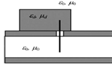
Figure 6. Waveguide-probe-excited circular disk DRA [35].
