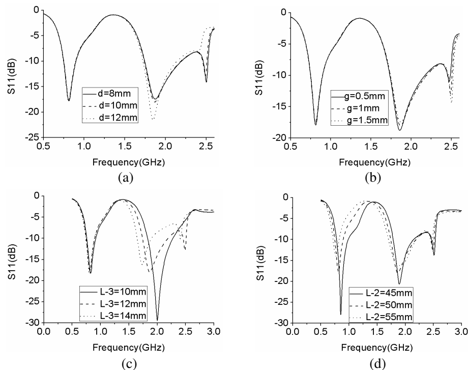
Figure 5. Simulated S_{11} of the proposed wideband monopole antenna, (a) variations in d , (b) variations in g , (c) variations in L_3 , (d) variations in L_2 .
