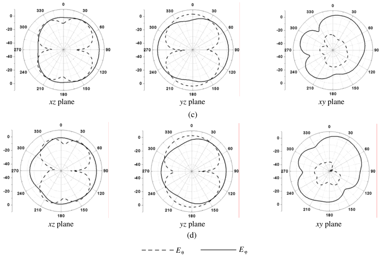
Figure 8. Measured radiation patterns of the fabricated antenna (co-polarization and cross-polarization) of the proposed antenna at different frequencies, (a) 740 MHz, (b) 1795 MHz, (c) 2.1 GHz and (d) 2.45 GHz.
