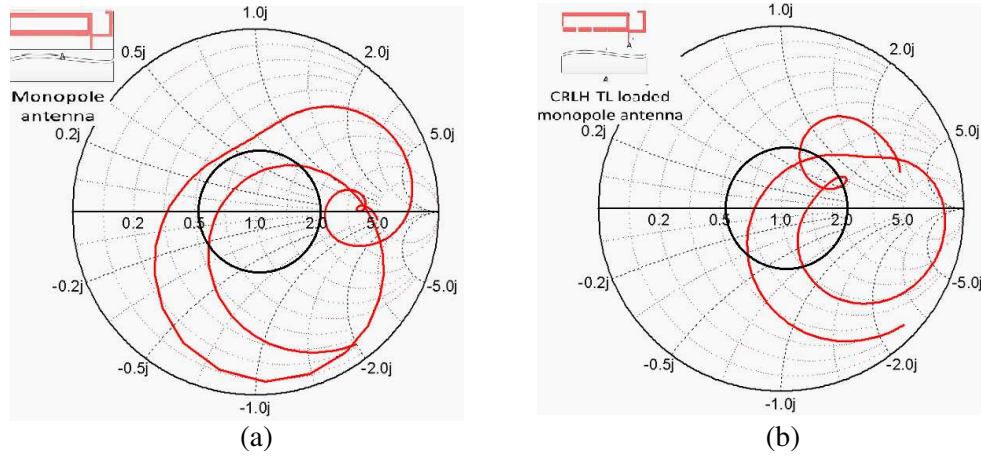
Figure 3. Simulated input impedance from 0.5 GHz to 3 GHz for (a) monopole antenna, (b) CRLH-TL loaded monopole antenna.
