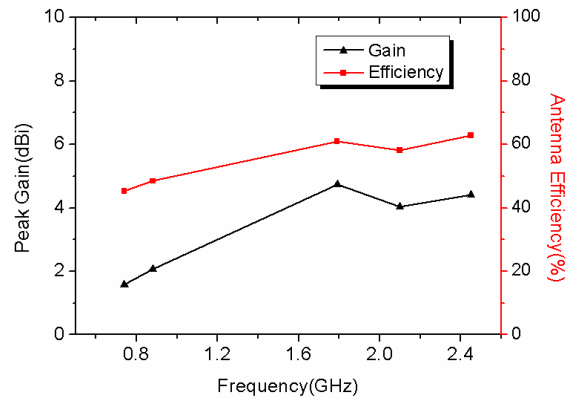
Figure 9. Gain and efficiency of the proposed antenna.
