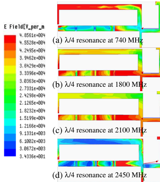
Figure 4. Surface currents on proposed monopole antenna with RLH-TL at (a) 740 MHz, (b) 1800 MHz, (c) 2100 MHz, (d) 2450 MHz.
