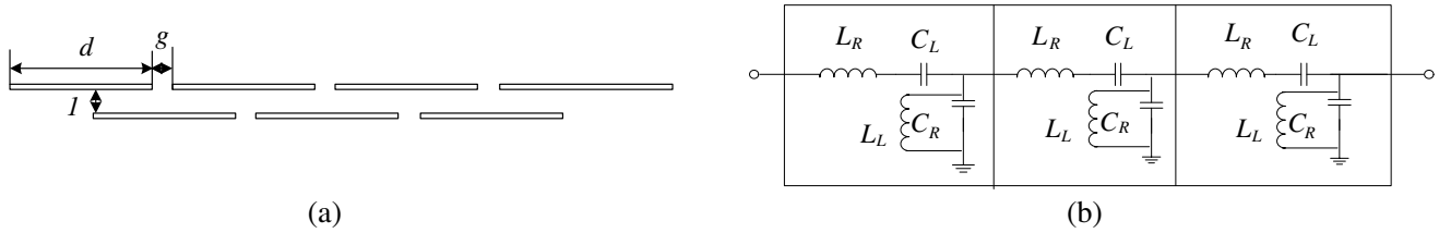
Figure 1. (a) Side view of the presented parallel-plate lines. (b) Corresponding equivalent lumped-element circuit model.
