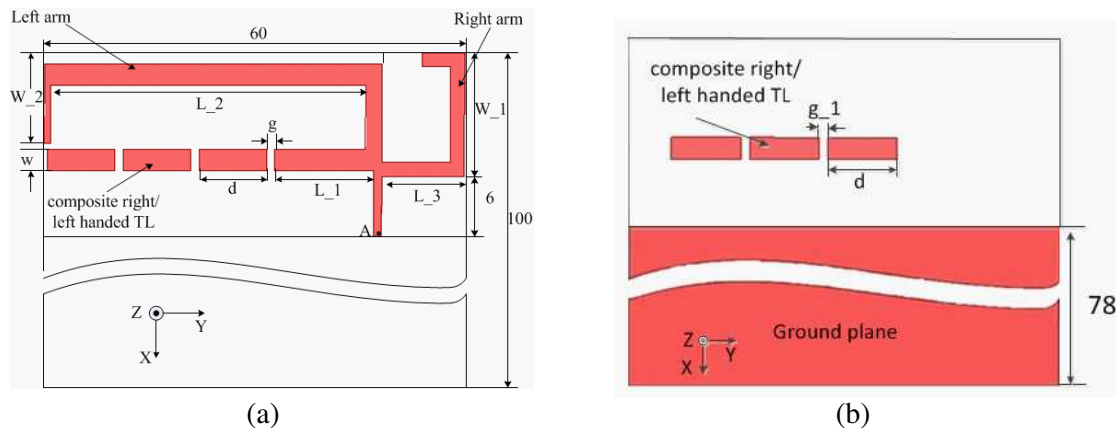
Figure 2. (a) Top view, (b) bottom view of the proposed wideband CRLH-TL monopole antenna.
