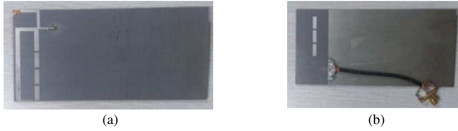
Figure 6. Prototype of the proposed multiband antenna, (a) top view, (b) back view.
