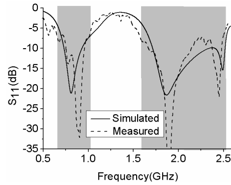
Figure 7. Measured and simulated S_{11} of the proposed antenna.
