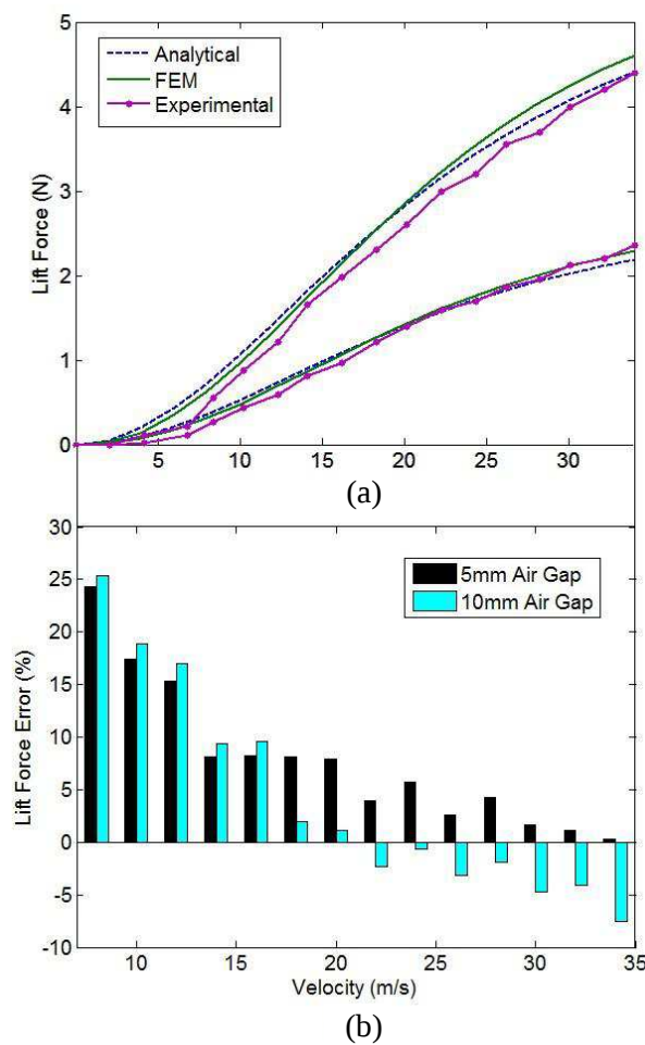
Figure 13. Lift force; (a) Value, (b) error.
