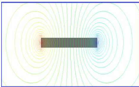
Figure 8. Magnetic flux paths around the PM.
