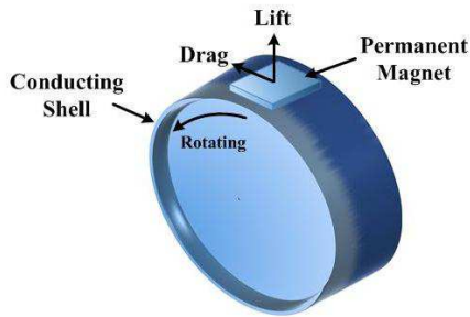
Figure 6. Schematic view of PEDS system.
