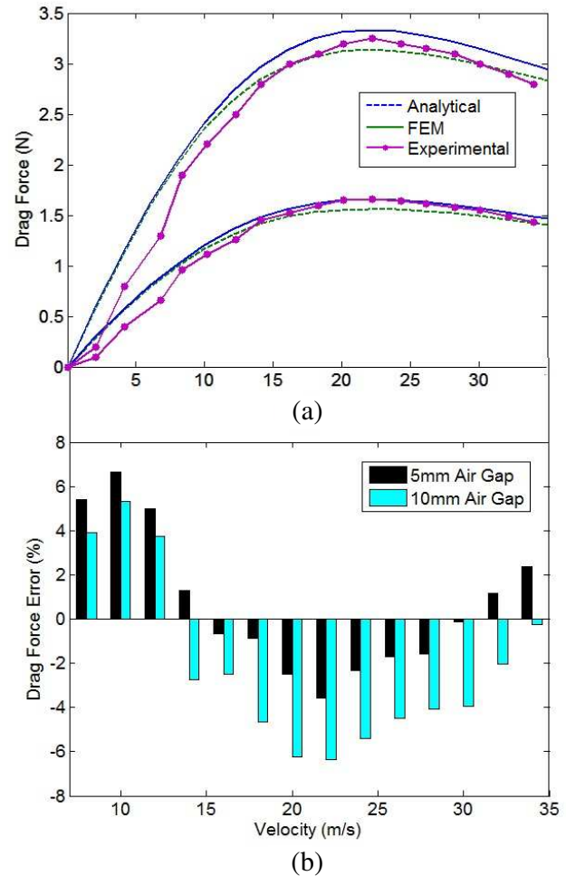
Figure 14. Drag force; (a) Value, (b) error.
