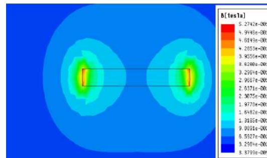
Figure 9. Magnetic field spectrum around the PM.
