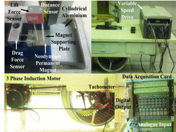
Figure 11. Experimental PEDS system.
