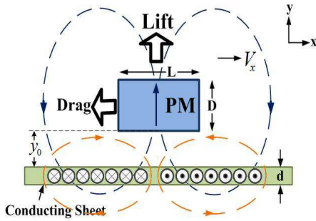
Figure 1. Physical model of electro-dynamic suspension system.
