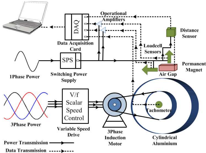
Figure 12. Schematic view of experimental system.
