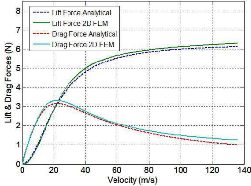
Figure 10. Lift and drag forces in terms of velocity.
