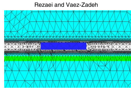
Figure 7. Mesh generation of PEDS model.
