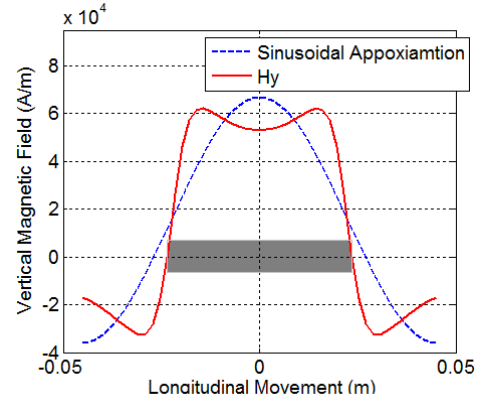
Figure 4. Vertical magnetic field and its fundamental component.
