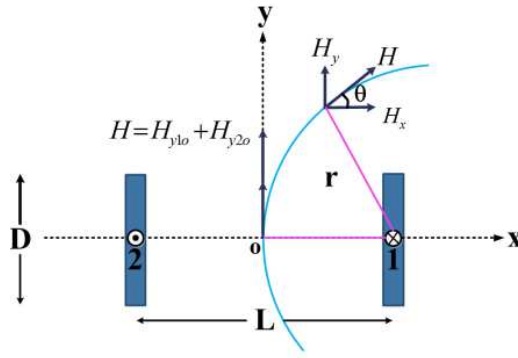
Figure 5. Model of PM by single current sheet.
