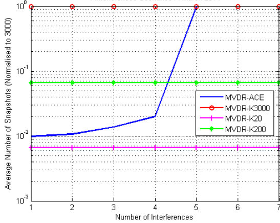
Figure 7. Scenario A: average number of snapshots for MVDR-ACE, MVDR-K3000, MVDR-K200 and MVDR-K20 beamformers.
