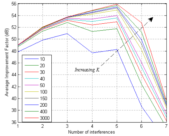
Figure 4. Scenario B: average improvement factor versus the number of interferences for MVDR-SMI at various snapshot sizes, K .
