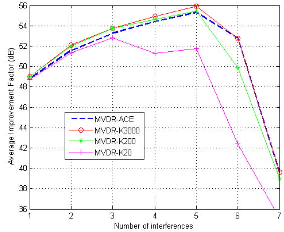
Figure 6. Scenario B: average improvement factor for MVDR-ACE, MVDR-K20, MVDR-K200 and MVDR-K3000 beamformers.
