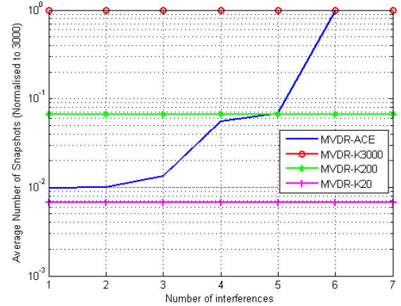
Figure 8. Scenario B: average number of snapshots for MVDR-ACE, MVDR-K3000, MVDR-K200 and MVDR-K20 beamformers.
