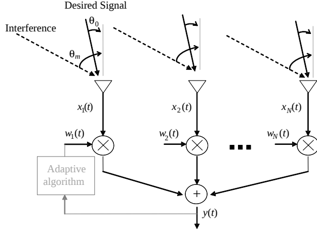
Figure 1. Block diagram of an N -element adaptive array.
