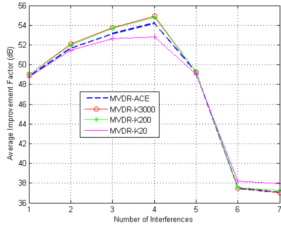
Figure 5. Scenario A: average improvement factor for MVDR-ACE, MVDR-K20, MVDR-K200 and MVDR-K3000 beamformers.
