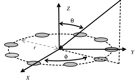
Figure 2. Geometry structure of a uniform N -element circular array.
