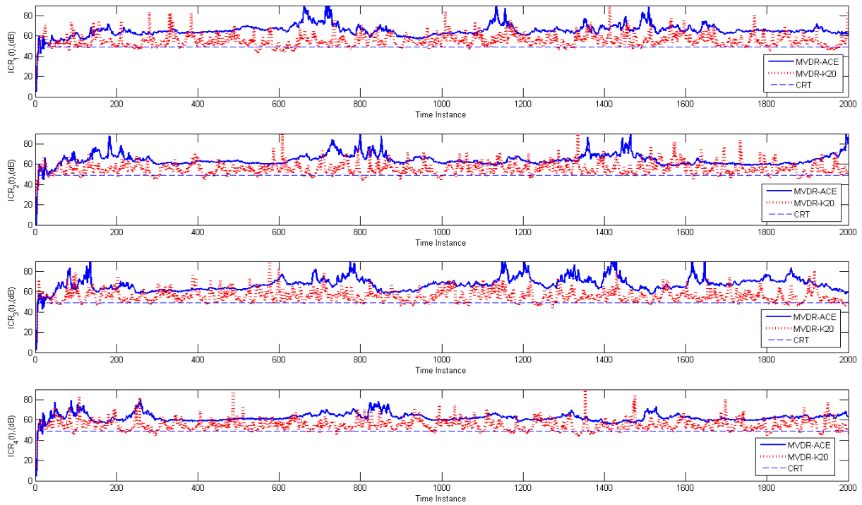
Figure 10. Scenario B, four interferences case: instantaneous cancellation ratio on all the four interferences of MVDR-ACE and MVDR-K20 beamformer.
