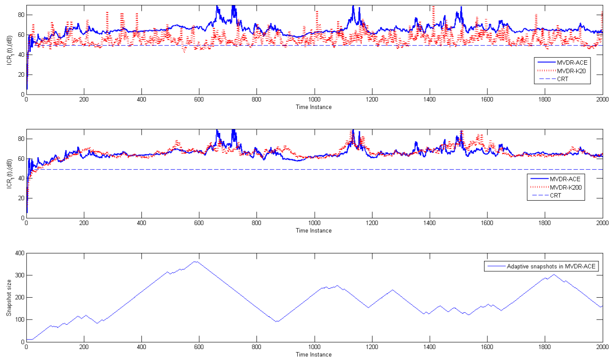
Figure 9. Scenario B, four interferences case: instantaneous cancellation ratio on interference ( 80^\circ, 0^\circ ) of MVDR-ACE, MVDR-K20 and MVDR-K200. The snapshot variation of the MVDR-ACE beamformer is included.
