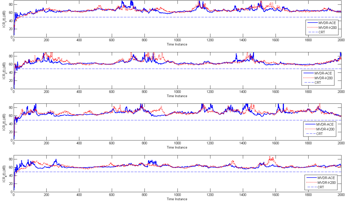
Figure 11. Scenario B, four interferences case: instantaneous cancellation ratio on interference on all the four interferences of MVDR-ACE and MVDR-K200 beamformer.
