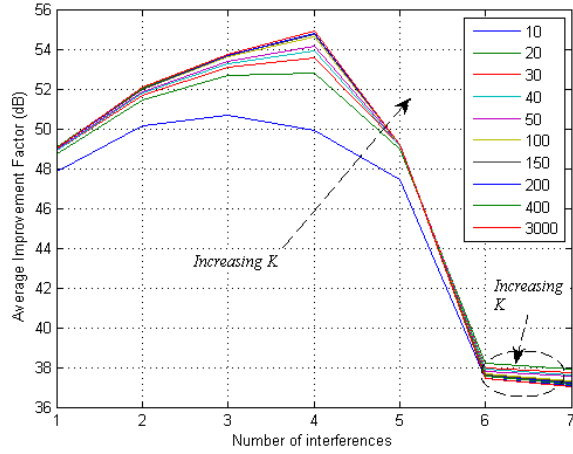
Figure 3. Scenario A: average improvement factor versus the number of interferences for MVDR-SMI at various snapshot sizes, K .
