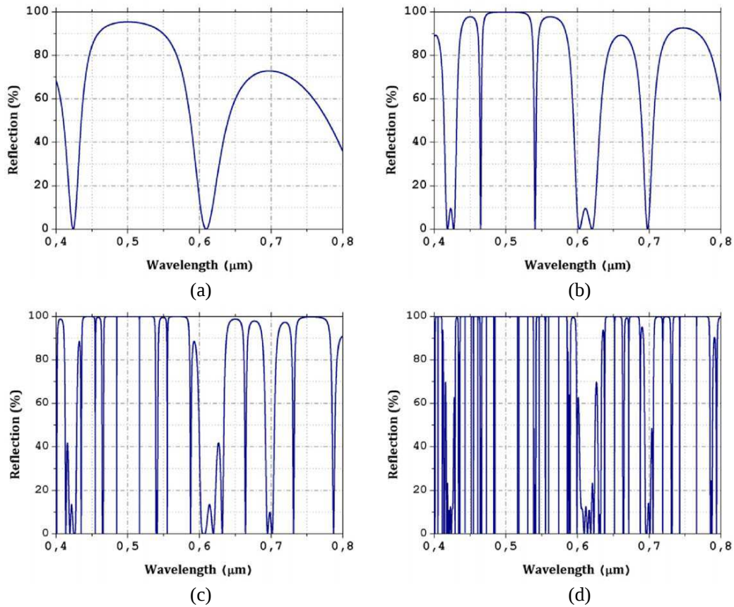
Figure 3. Spectra reflections of quasi-periodic multilayer structures according to the Triadic-Cantor distribution for different iterations: (a) 2nd iteration, (b) 3rd iteration, (c) 4th iteration, (d) 5th iteration.
