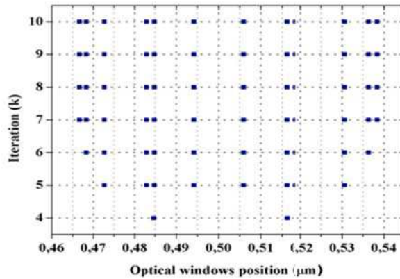
Figure 6. Number and position of the optical windows according to the iteration number ( k ).
