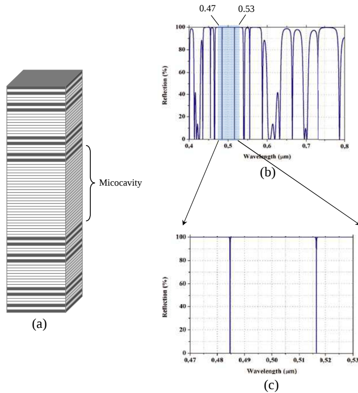
Figure 7. (a) The configuration of a multilayer structure according to the Triadic-Cantor distribution for the 4th iteration, (b) reflection spectrum of a multilayer structure according to Triadic-Cantor distribution between 0.4 \mu\text{m} and 0.8 \mu\text{m} , (c) reflection spectrum of a multilayer structure according to Triadic-Cantor distribution between 0.47 \mu\text{m} and 0.53 \mu\text{m} .
