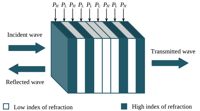
Figure 2. The one-dimensional multilayer dielectric structure according to the Triadic-Cantor distribution for the 2nd iteration ( HLHLLLHLH ).
