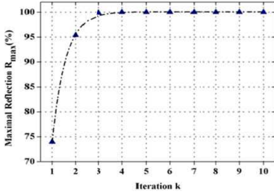
Figure 4. The maximal reflection R_{\max} (%) Variation according to the iteration number ( k ).
