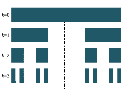
Figure 1. The Triadic-Cantor set presentation for iteration: k = 0 , k = 1 , k = 2 and k = 3 .
