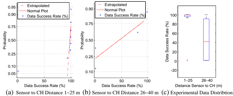
Figure 4. Analysis of experimental data in a multi storey building: normal probability values. (a) Distance 1–25 m. (b) Distance 26–40 m. These values are computed from the formula explained in the Section 4.1. (c) Data success rate for different distance between the sensor to CH.
