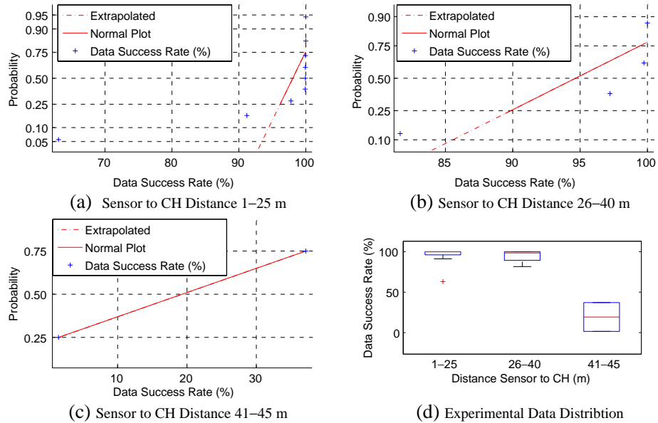
Figure 3. Analysis of experimental data in a single storey building: Normal probability values. (a) Distance 1–25 m. (b) Distance 26–40 m. (c) Distance 41–45 m. These values are computed from the formula explained in the Section 4.1. (d) Data success rate for different distance between the sensor to CH.
