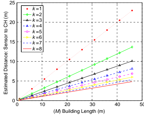
Figure 2. The mean square distance from the sensor to the CH versus building length M with different number of k clusters. This shows the difference between the building length and the number of clusters does have significant effect to the estimation of the distance between from the sensor to the CH.
