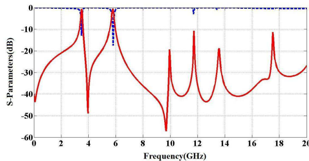
Figure 4. S -parameters of the optimized filter.
