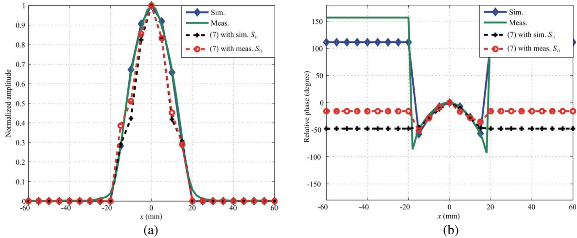
Figure 6. Electric near-field distribution at AUT aperture: (a) normalized amplitude; (b) relative phase.
