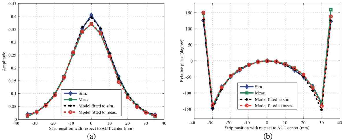
Figure 5. Simulated and measured S_{11} : (a) amplitude; (b) relative phase.
