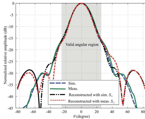
Figure 7. Normalized far-field pattern at 30 GHz.
