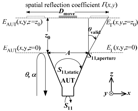
Figure 1. Schematic layout of the proposed antenna pattern retrieval method.
