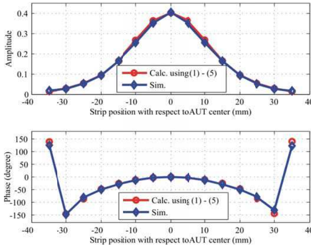
Figure 3. The comparison of reflection coefficient calculated using Eqs. (1)–(5) and obtained from simulator.
