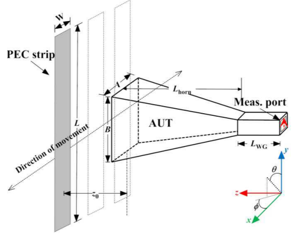
Figure 2. Simulation setup and the pyramidal horn dimensions (not to scale).
