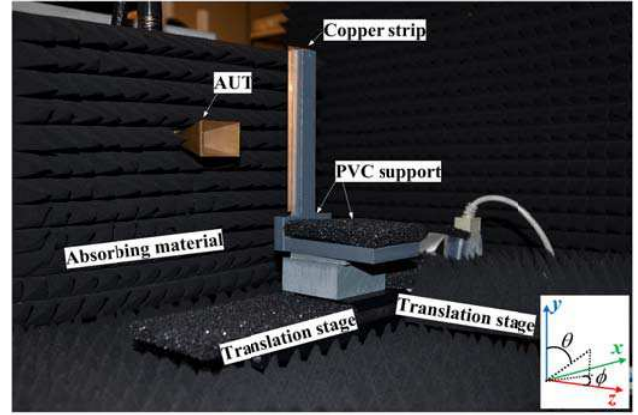
Figure 4. Photograph of the experimental setup.
