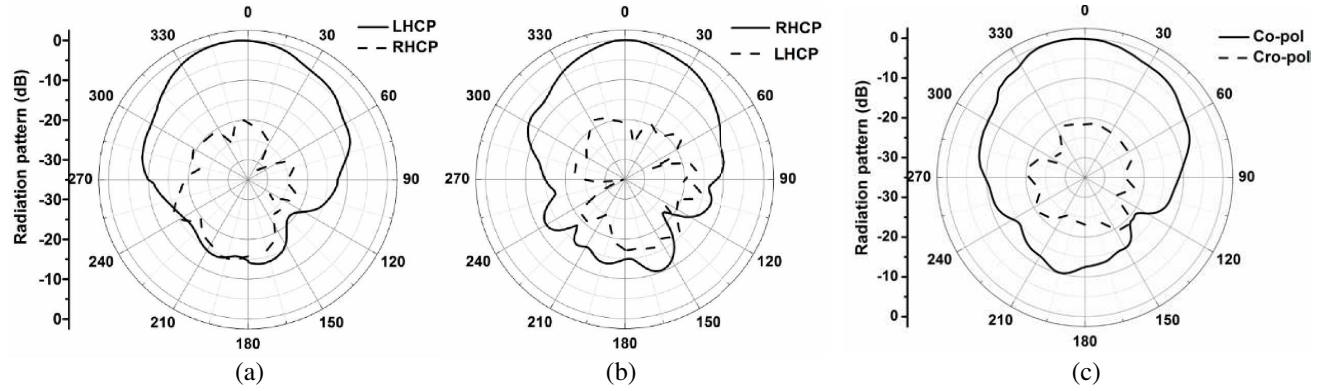
Figure 12. Measured radiation patterns of the proposed reconfigurable antenna. (a) LHCP, (b) RHCP, and (c) LP.
