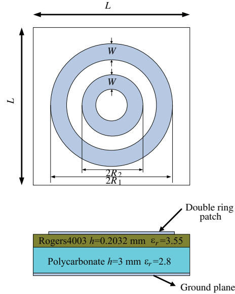
Figure 1. Geometry of the double concentric circular ring element.
