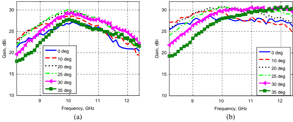
Figure 8. Measured gain of the reflectarrays when the beam is scanned (a) \lambda/2 grid spacing and (b) 0.3\lambda grid spacing.
