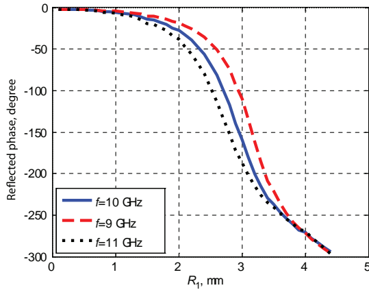
Figure 2. Reflected phase curves of the double concentric circular ring element with 0.3\lambda (9 mm) grid and ring spacing of R_2 = 0.53R_1 for different frequencies.
