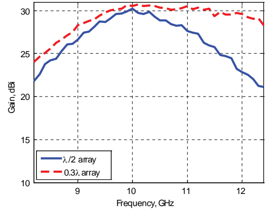
Figure 5. Measured gain of two reflectarrays.
