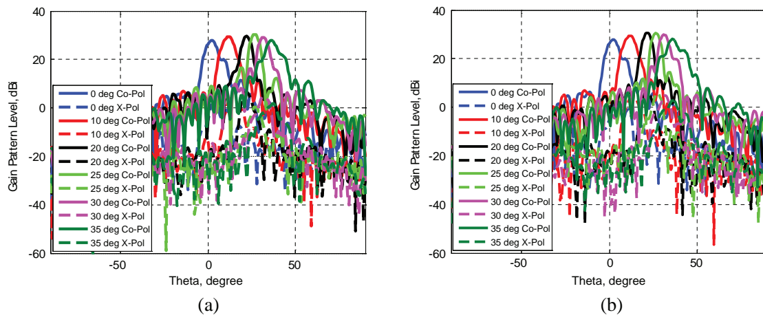
Figure 7. Measured scanned beam patterns of the reflectarray with (a) \lambda/2 grid spacing and (b) 0.3\lambda grid spacing at 10GHz.
