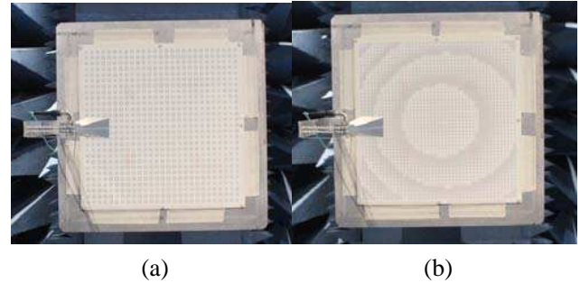
Figure 3. Prototypes of the reflectarrays, (a) \lambda/2 array with 729 double concentric circular rings, (b) 0.3\lambda array with 2025 double concentric circular rings.
