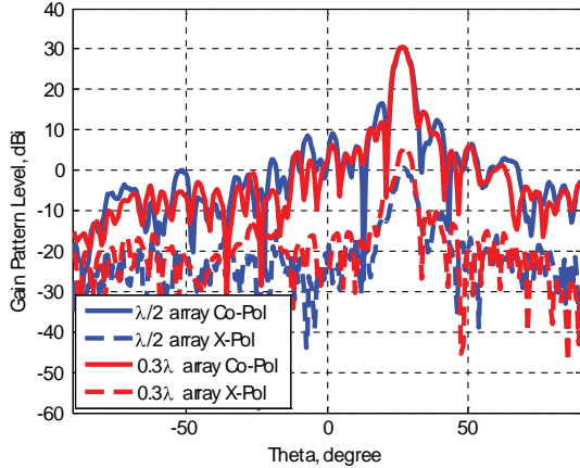
Figure 4. Measured E -plane radiation patterns at 10 GHz for two reflectarrays.
