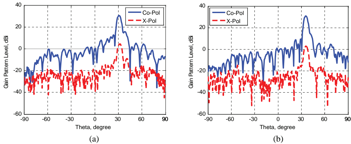
Figure 10. Measured E -plane radiation patterns of the 0.3\lambda reflectarray with (a) scan angle of 30^\circ at 11 GHz and (b) scan angle of 35^\circ at 12.9 GHz.
