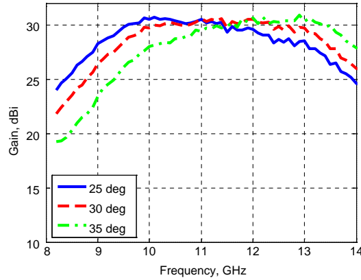
Figure 9. Measured gain of the 0.3\lambda reflectarray with scan angles of 25°, 30° and 35°.
