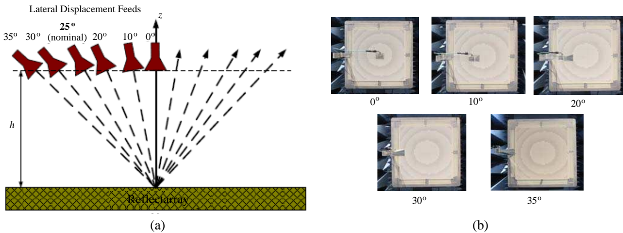
Figure 6. (a) Lateral displacement of feeds and (b) prototypes of the 0.3\lambda reflectarray with lateral displaced feeds.
