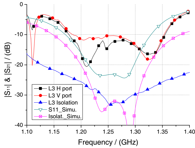
Figure 8. Measured and simulated L-band element |S_{11}| .
