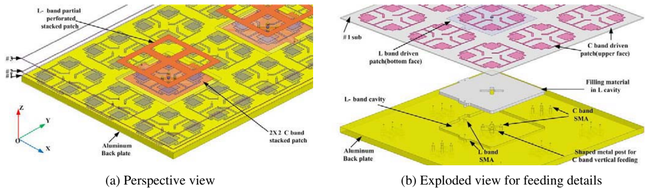
Figure 4. Configuration of sandwiched DBDP sub array.
