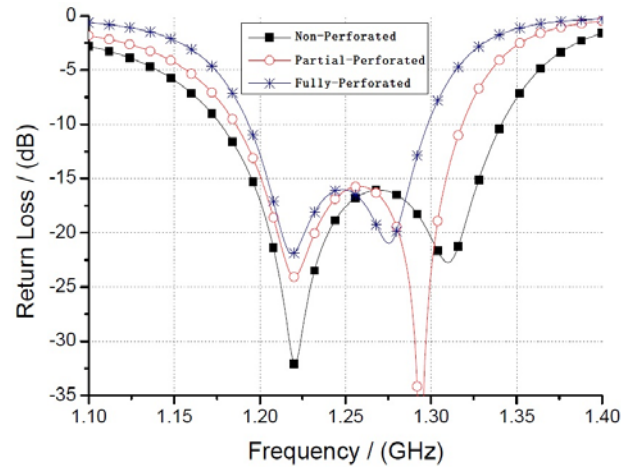
Figure 2. Relationship between bandwidth and perforation.
