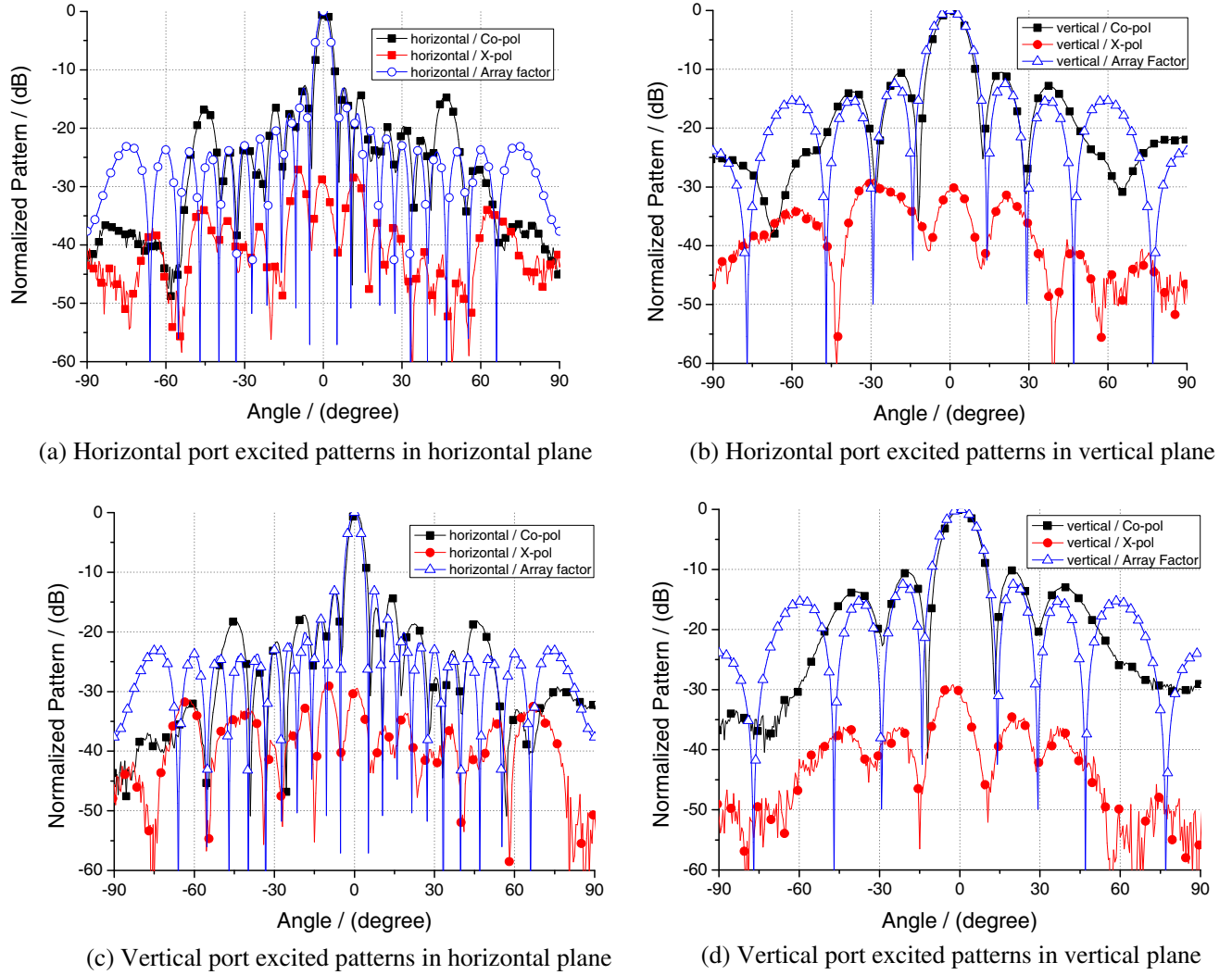
Figure 11. Measured and calculated C-band radiation pattern at 5.8 GHz.
