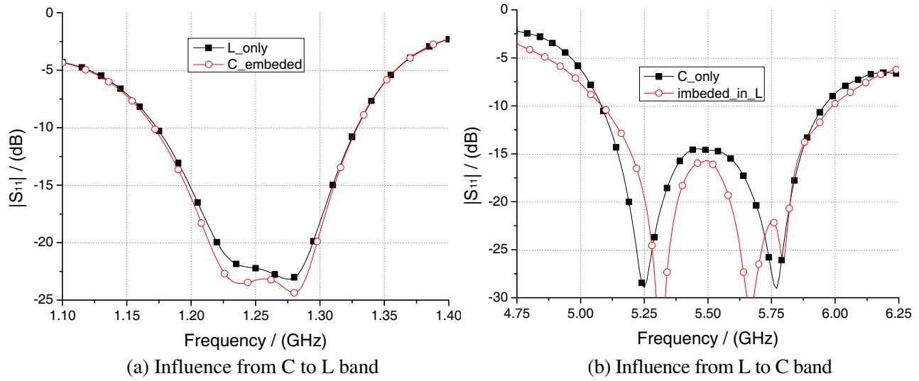
Figure 6. Influence from inter-band coupling.
