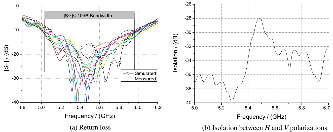
Figure 10. Measured and simulated C-band element port response.
