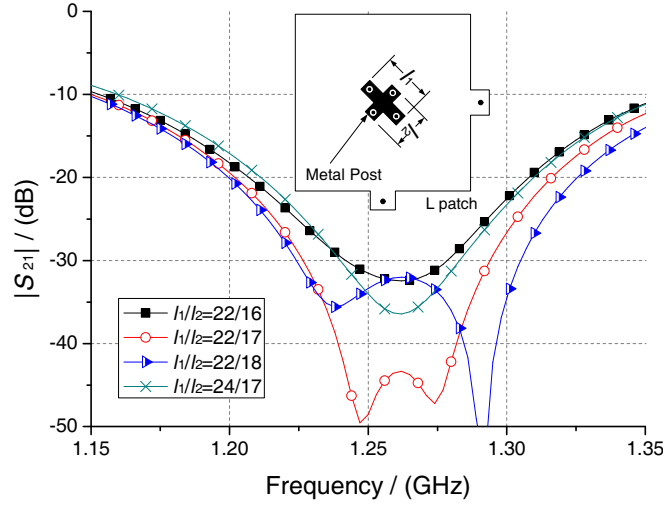
Figure 5. Parameter study on metal post shape and isolation.
