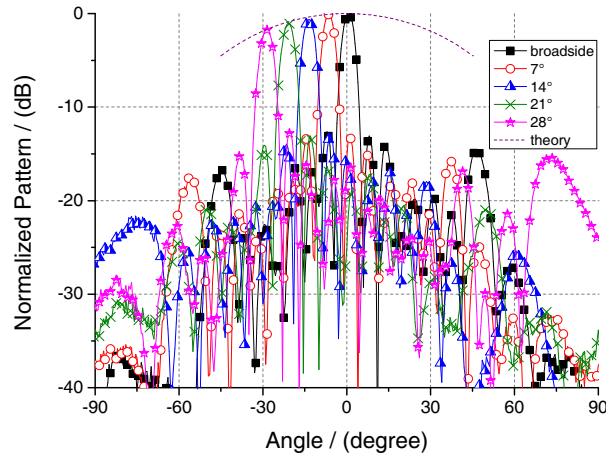
Figure 12. Simulated C-band scan radiation pattern at 5.8 GHz.
