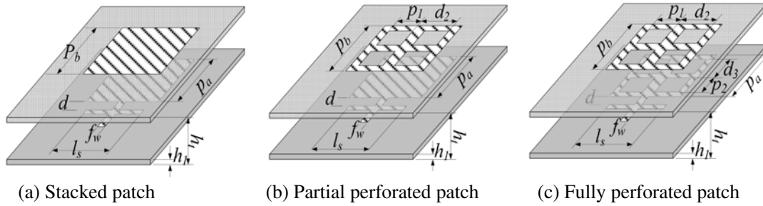
Figure 1. Configurations of stacked patch with different perforation.
