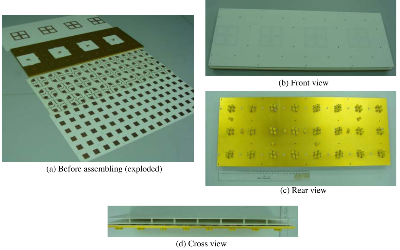
Figure 7. Photos of sandwiched stacked patch DBDP array.
