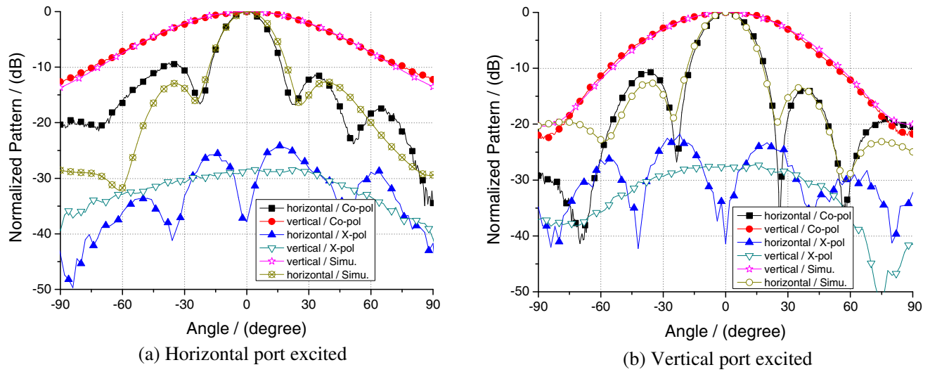
Figure 9. Measured and simulated L-band radiation pattern at 1.25 GHz.
