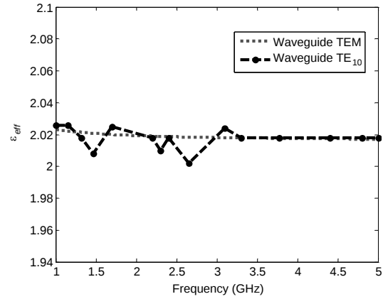
Figure 6. Comparison of \epsilon_{eff} for TE_{10} and TEM waveguide tests.
