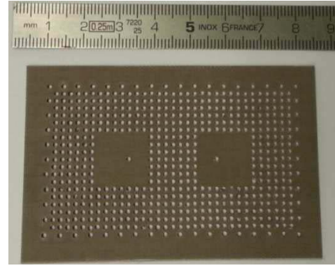
Figure 9. Photograph of the drilled substrate of the SINRD filter (order 2).
