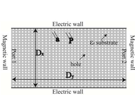
Figure 2. SINRD waveguide of fundamental mode TE 10 .
