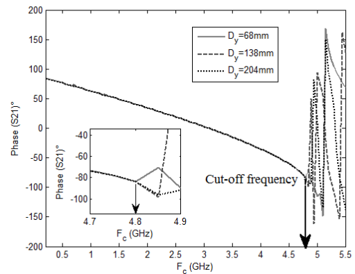
Figure 3. Phase of S_{21} for several distances by between ports.
