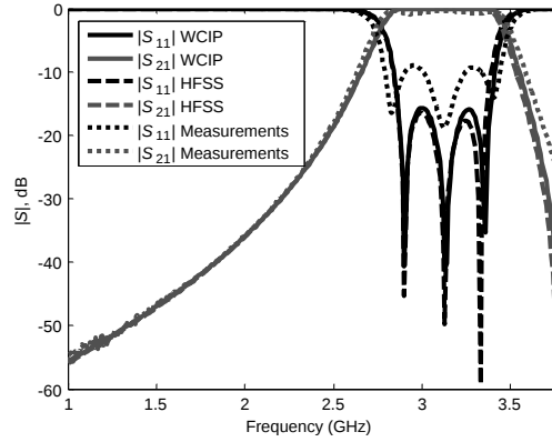
Figure 13. S -parameters of the filter of Fig. 12.
