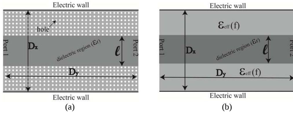
Figure 7. Dielectric waveguide structures for (a) WCIP, (b) equivalent waveguide for HFSS.
