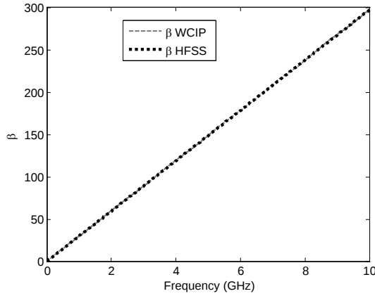
Figure 5. Propagation constant \beta versus frequency.
