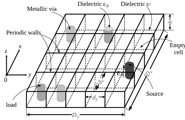
Figure 1. Substrate integrated circuit example.
