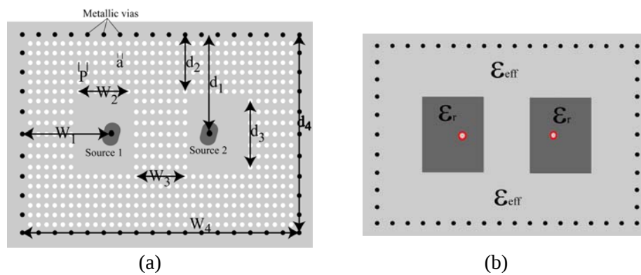
Figure 10. (a) SINRD filter of 2nd order, (b) equivalent homogeneous filter for HFSS simulation.
