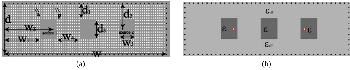
Figure 12. (a) SINRD filter of 3rd order, (b) equivalent homogeneous filter for HFSS simulation.
