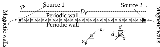
Figure 4. SINRD waveguide of fundamental mode TEM.
