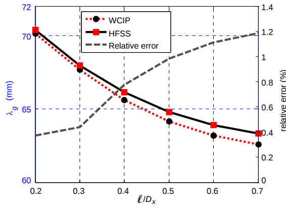
Figure 8. Guided wavelength \lambda_g depending on \ell/D_x .
