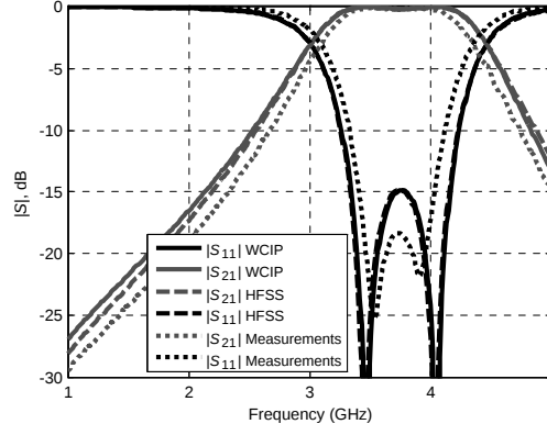
Figure 11. S -parameters of the filter of Fig. 10.
