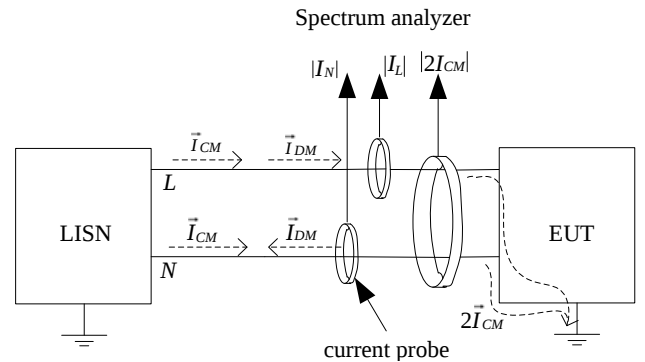
Figure 2. The measurement arrangement.
