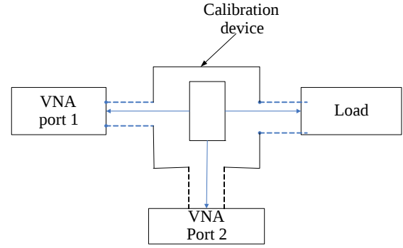
Figure 4. Calibration setup.
