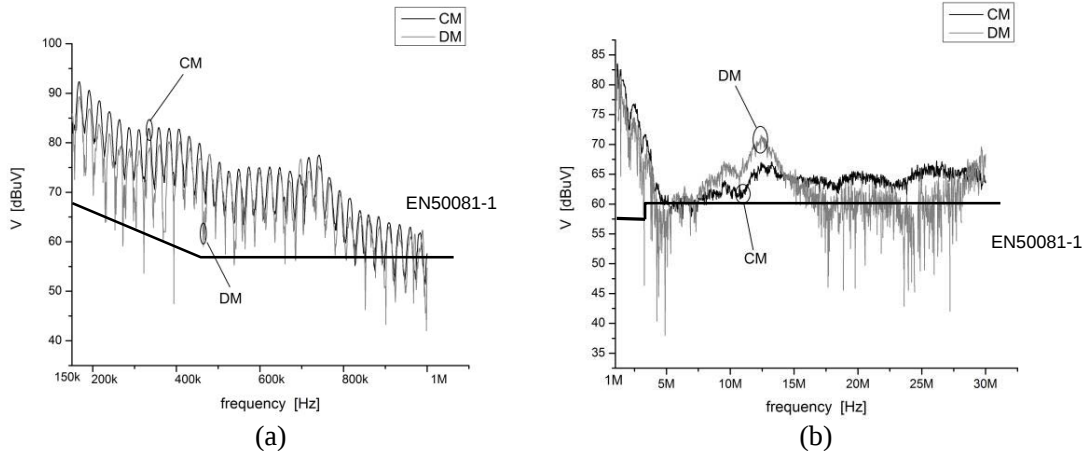
Figure 7. The CM and DM voltage spectrum at the frequency range, (a) from 150 kHz to 1 MHz, (b) from 1 MHz to 30 MHz.
