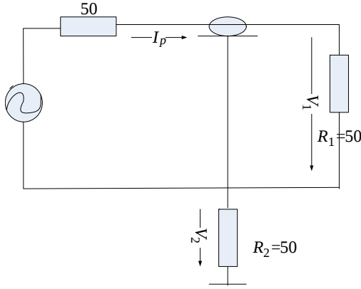
Figure 3. Schematic diagram.
