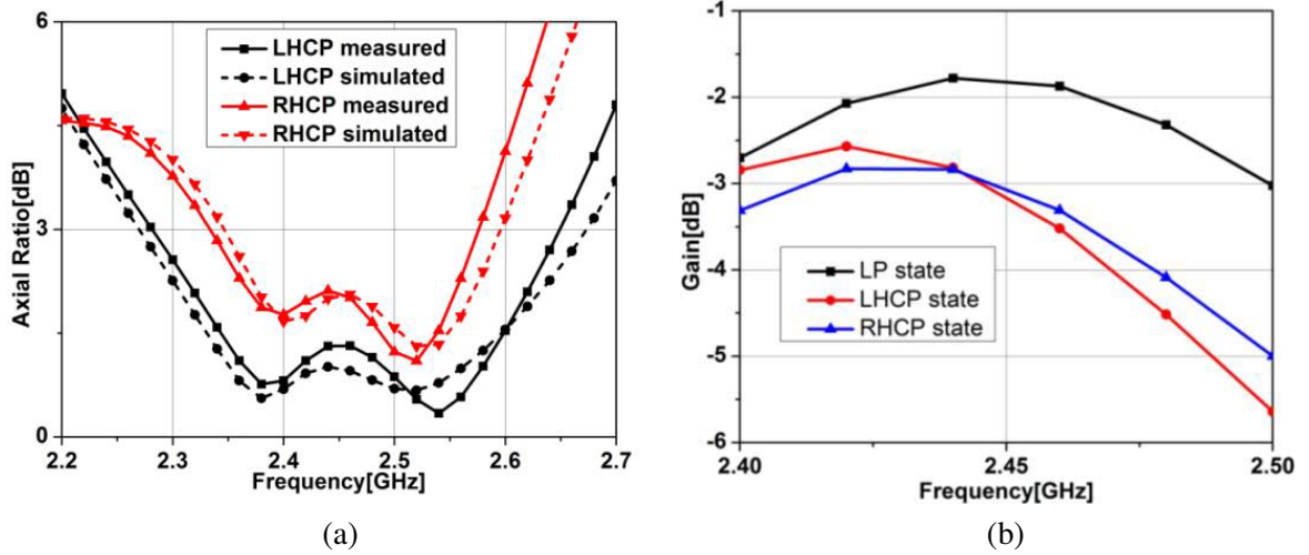
Figure 5. Comparison of axial ratio and gain: (a) simulated and measured axial ratio; (b) measured gain.
