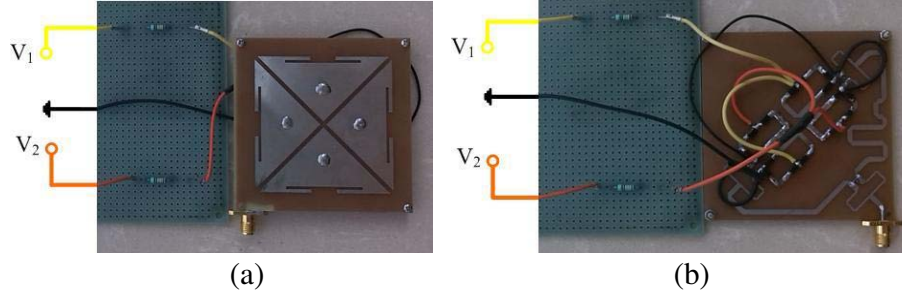
Figure 3. Antenna prototype: (a) top view; (b) bottom view.
