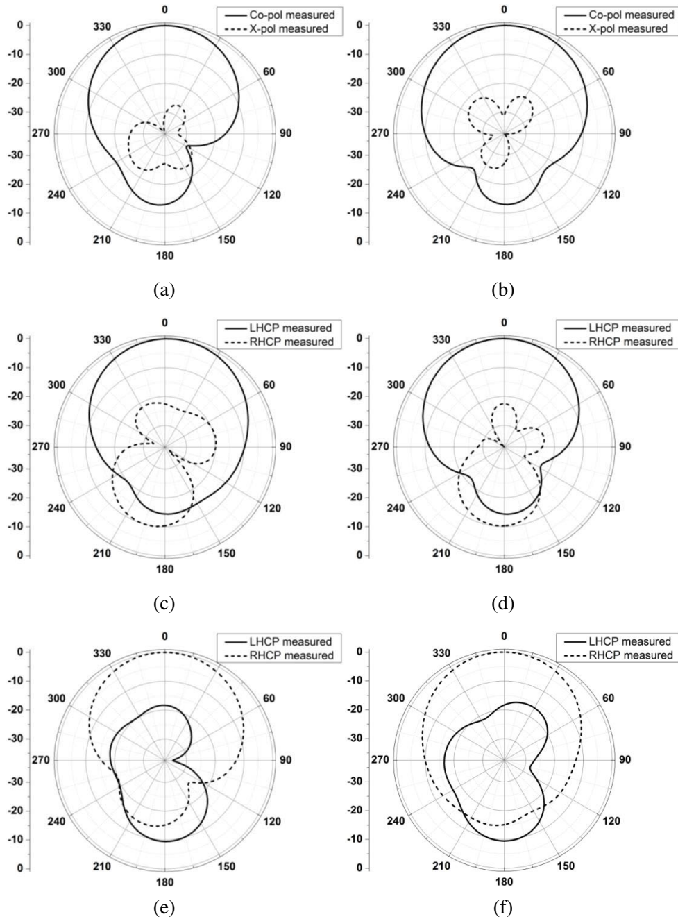
Figure 6. Radiation patterns on (a) \varphi = 45^\circ plane and (b) \varphi = -45^\circ plane for +45^\circ LP; (c) xoz -plane and (d) yo z -plane for LHCP; (e) xoz -plane and (f) yo z -plane for RHCP.
