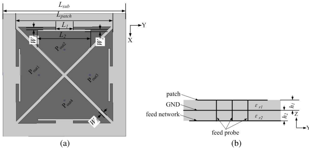
Figure 1. Geometry of the proposed antenna (a) top view and (b) side view.
