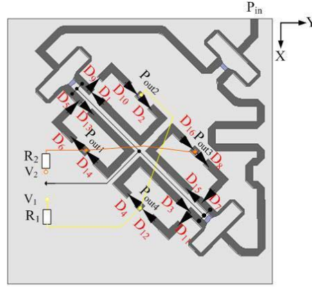
Figure 2. Feeding network and the associated dc biased network.
