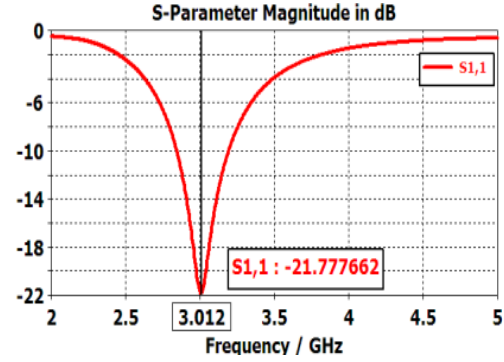
Figure 8. Simulation of return loss for the antenna with two cells of DGS.
