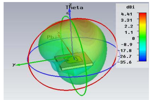
Figure 14. Radiation pattern for the conventional antenna.
